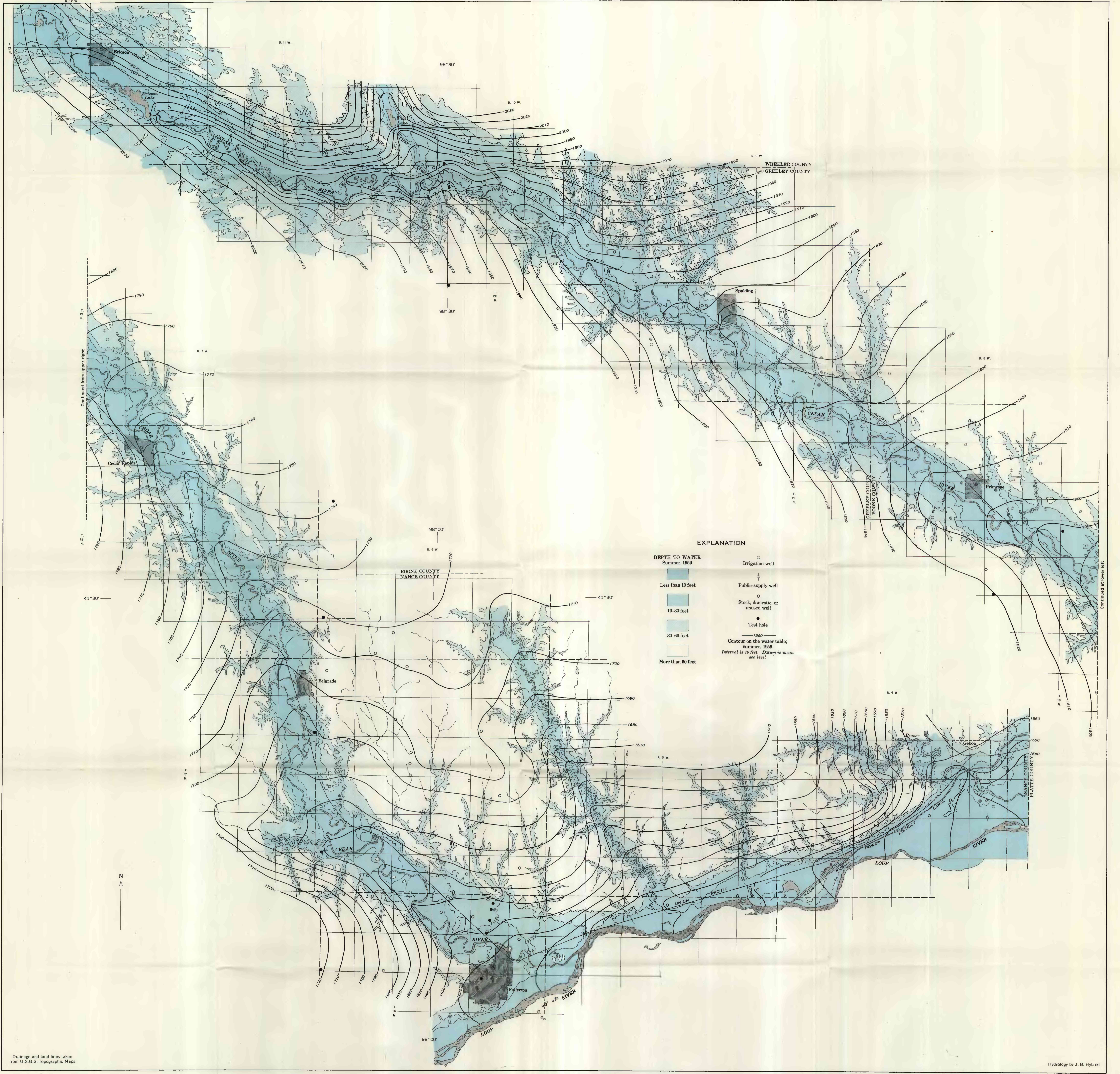
MAP SHOWING DEPTH TO WATER AND CONFIGURATION OF THE WATER TABLE IN THE CEDAR RAPIDS DIVISION PROJECT AREA, NEBRASKA
