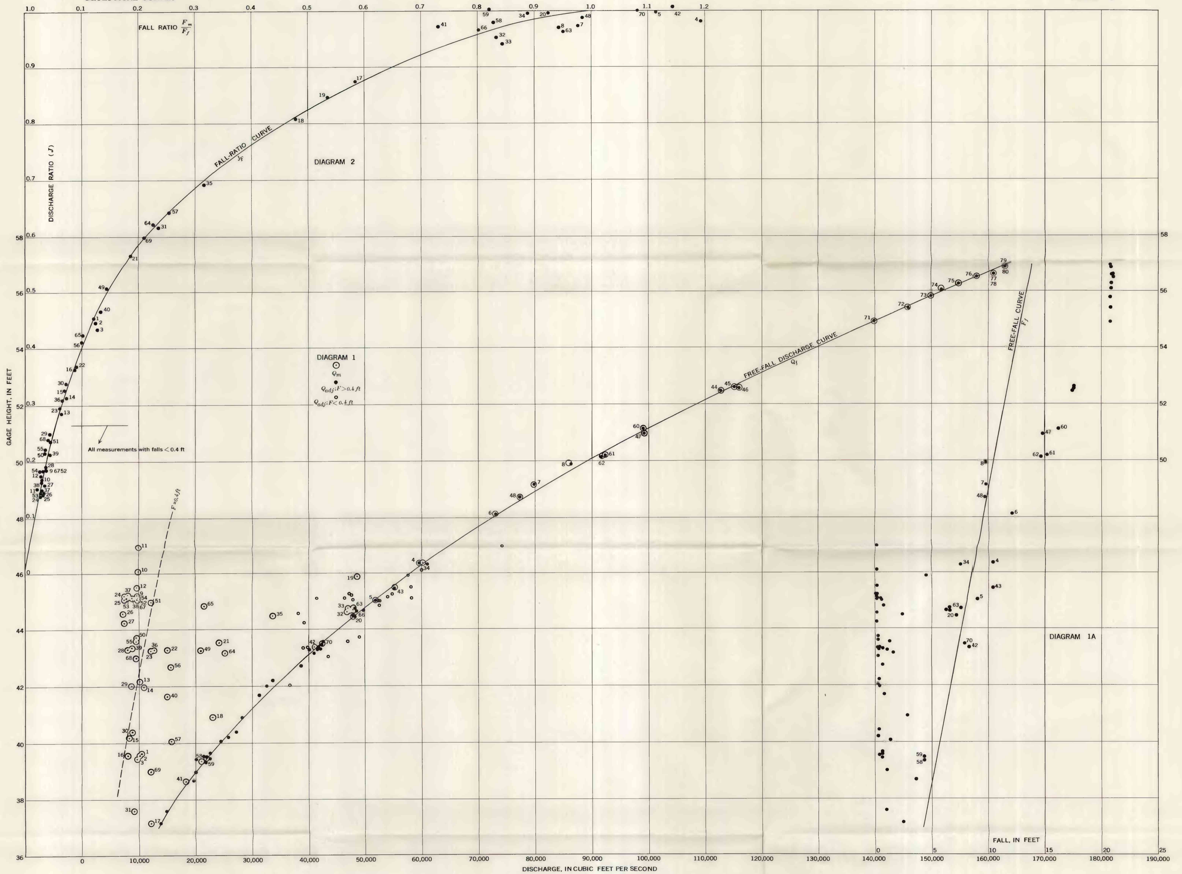
RELATION CURVES FOR RATING OF KOOTENAY RIVER AT GROHMAN, BRITISH COLUMBIA
