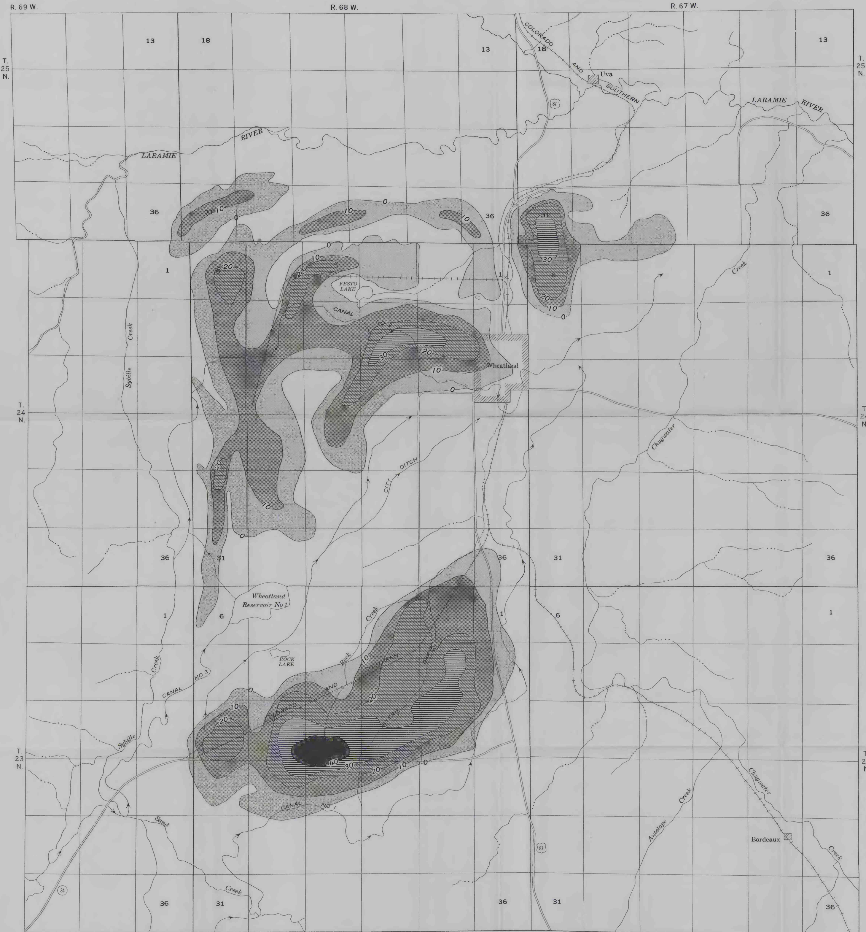
MAP OF THE WHEATLAND FLATS AREA, PLATTE COUNTY, WYOMING, SHOWING THE THICKNESS OF THE SATURATED PART OF THE TERRACE DEPOSITS, DECEMBER—JANUARY, 1959-60
