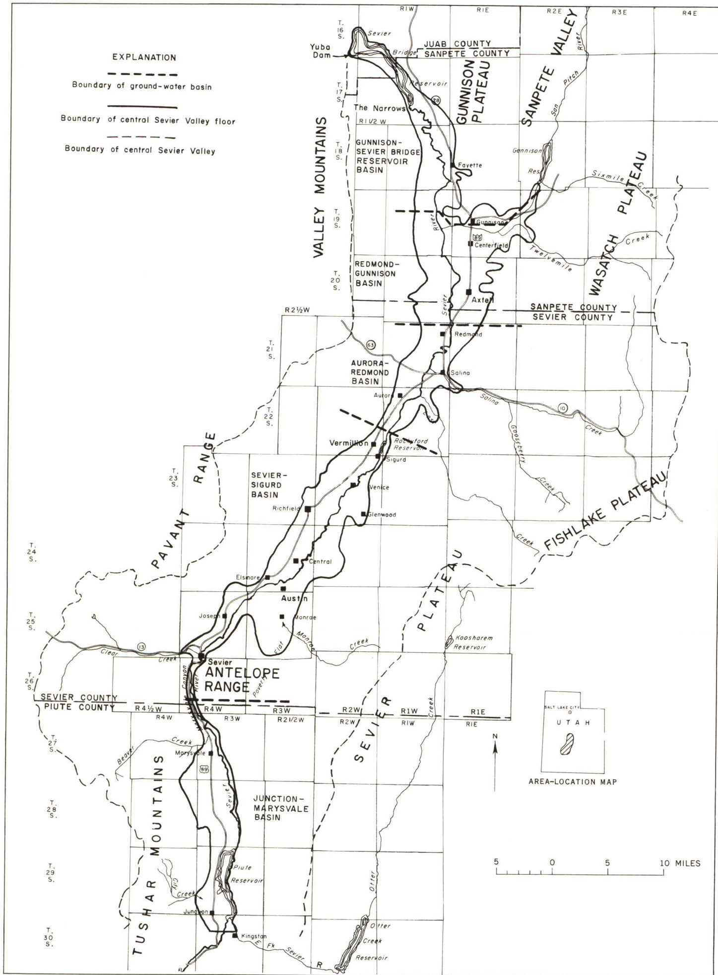
MAP OF PART OF CENTRAL UTAH SHOWING PHYSIOGRAPHIC SETTING AND GROUND-WATER BASINS OF THE CENTRAL SEVIER VALLEY
