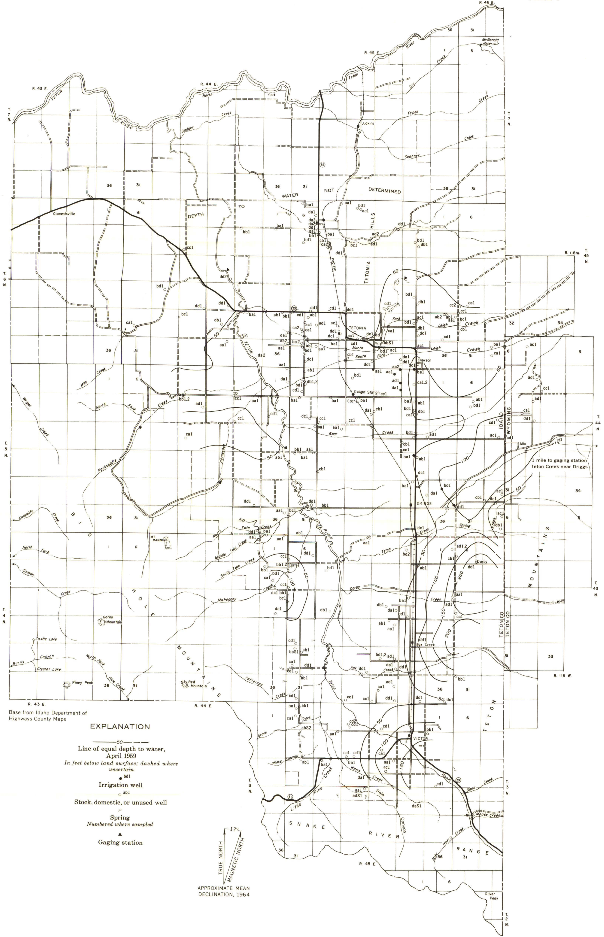
MAP SHOWING LOCATION OF WELLS, DEPTH TO WATER, AND OTHER HYDROLOGIC FEATURES IN THE UPPER TETON VALLEY, IDAHO AND WYOMING
