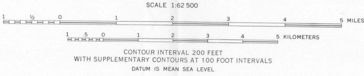
MAP SHOWING AREAS OF ARTESIAN FLOW AND PHREATOPHYTE OCCUPATION DURING 1960 IN PAVANT VALLEY, UTAH
