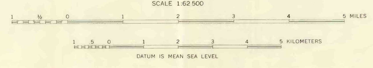
MAP SHOWING SURFACE GEOLOGY AND SECTIONS SHOWING SUBSURFACE GEOLOGY OF PORTAGE COUNTY, WISCONSIN
