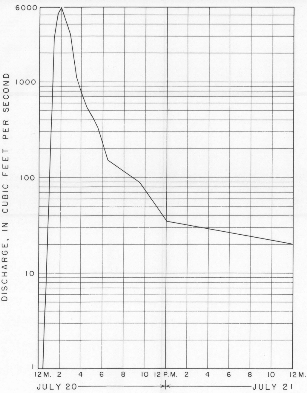
INFLOW AND OUTFLOW AT K-79 RESERVOIR NEAR EASTONVILLE, COLORADO, 1957
