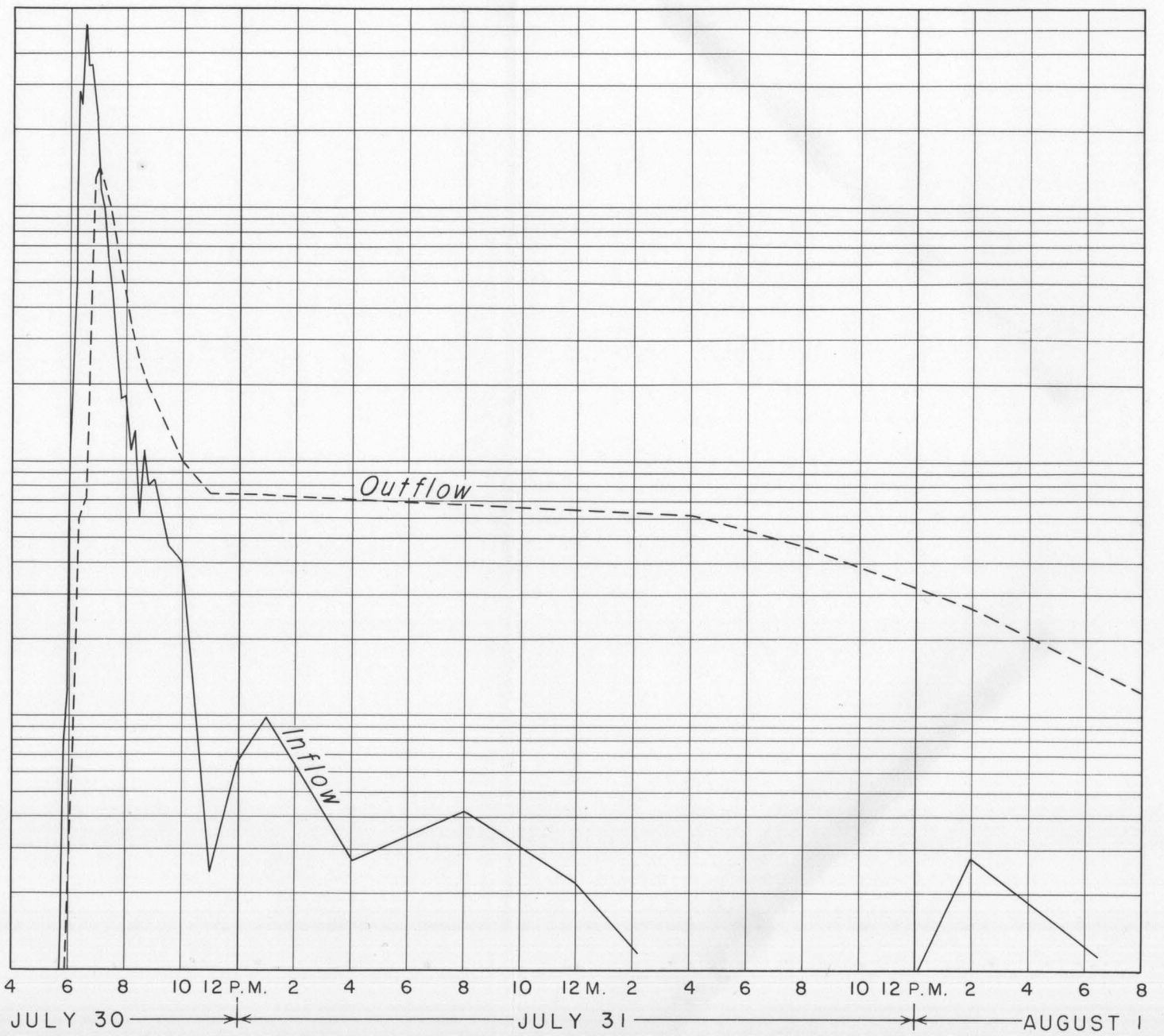
INFLOW AND OUTFLOW AT K-79 RESERVOIR NEAR EASTONVILLE, COLORADO, 1957
