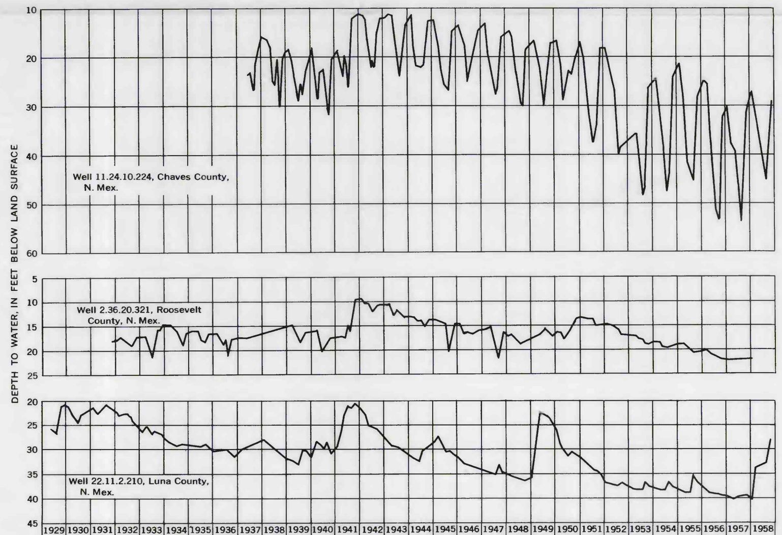
HYDROGRAPHS OF WELLS IN COLORADO, KANSAS, NEW MEXICO, AND TEXAS
