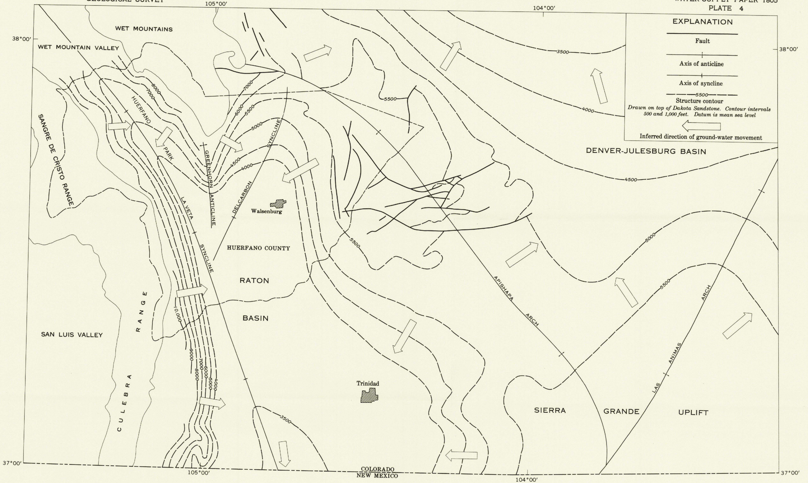
MAP OF PRINCIPAL STRUCTURAL FEATURES OF PART OF SOUTH-CENTRAL COLORADO
