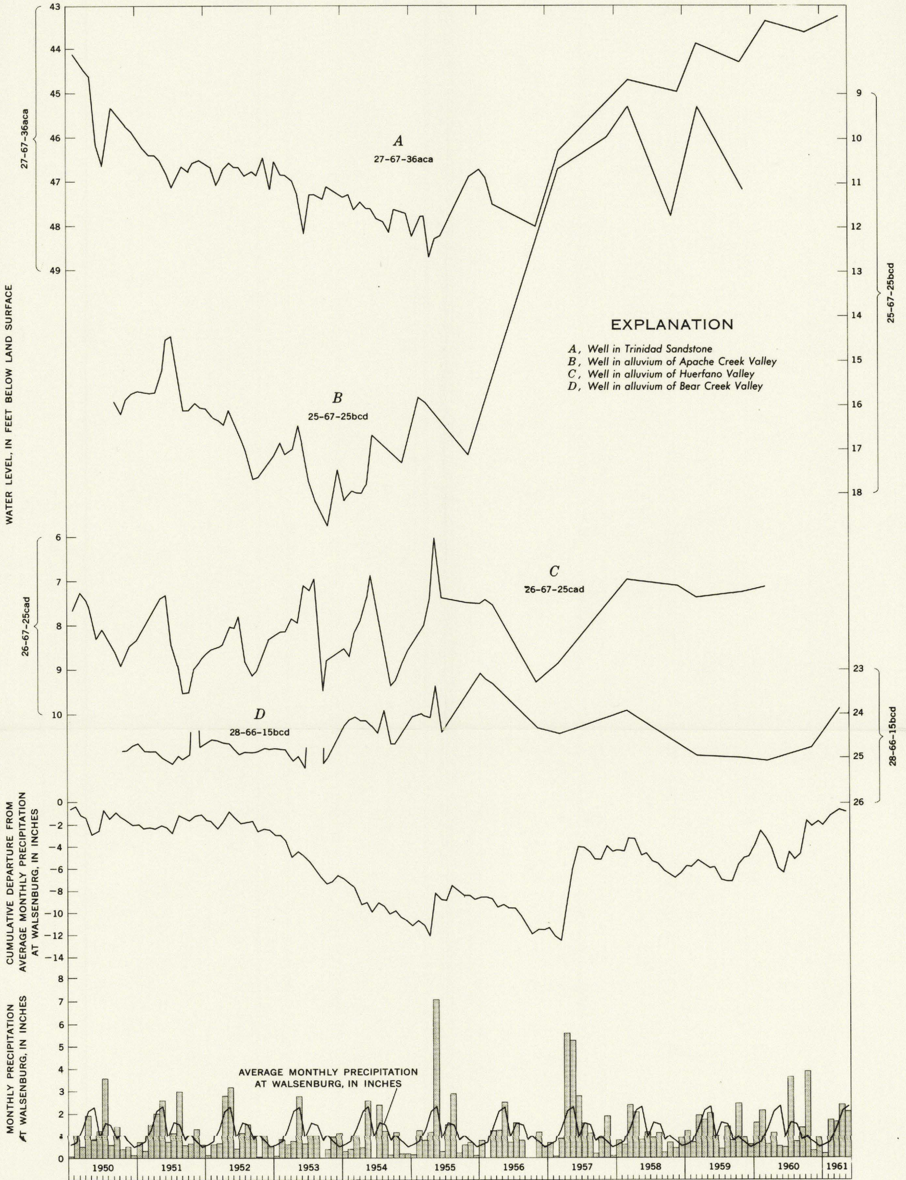
HYDROGRAPH OF WATER LEVEL IN OBSERVATION WELLS IN HUERFANO COUNTY AND PRECIPITATION AT WALSENBURG, COLORADO
