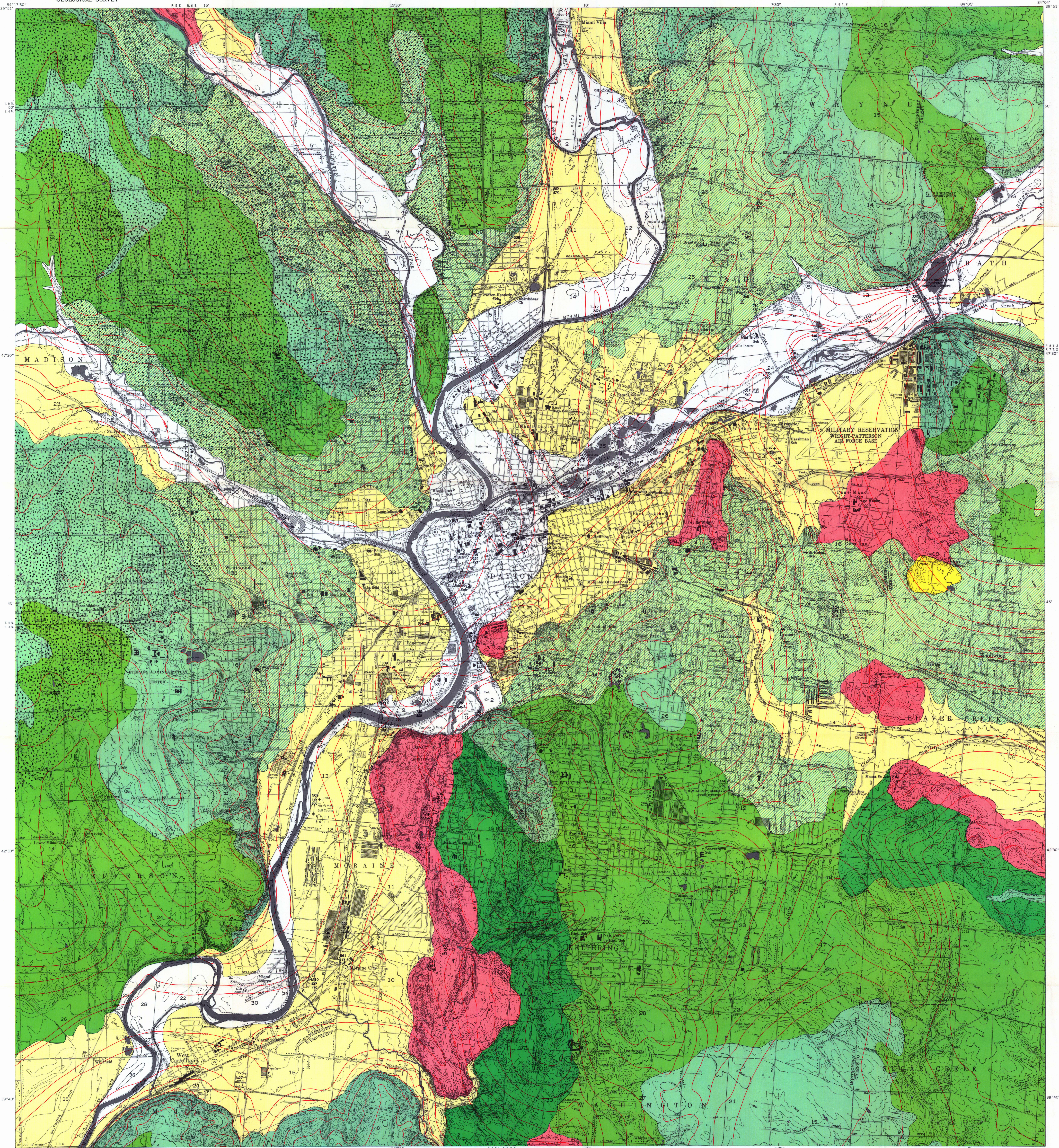
MAP OF THE DAYTON AREA, OHIO, SHOWING DISTRIBUTION OF THE GLACIAL AND ALLUVIAL DEPOSITS CONTOURS ON THE BEDROCK SURFACE, AND LOCATION OF GEOLOGIC SECTIONS
