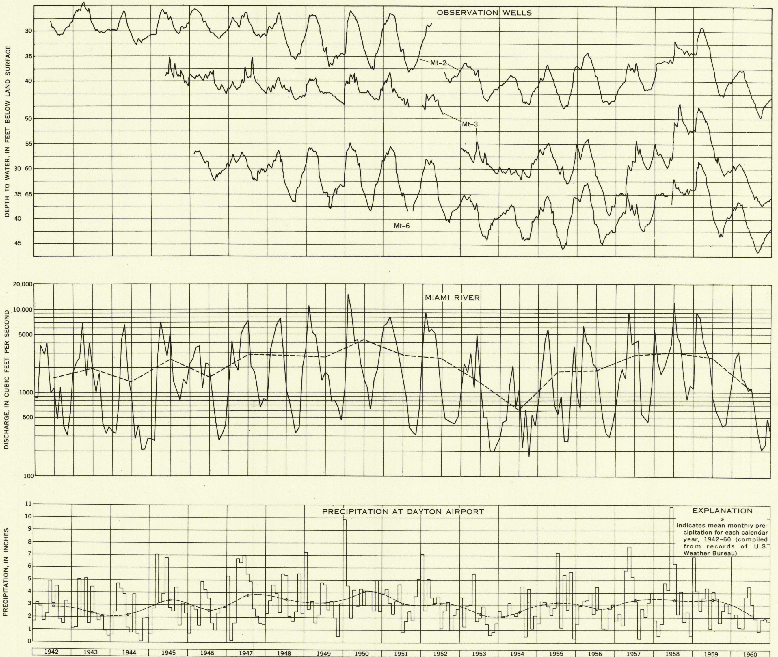
HYDROGRAPHS SHOWING WATER-LEVEL FLUCTUATIONS IN OBSERVATION WELLS, MEAN DISCHARGE OF MIAMI RIVER AT DAYTON, OHIO, AND MONTHLY PRECIPITATION AT DAYTON AIRPORT
