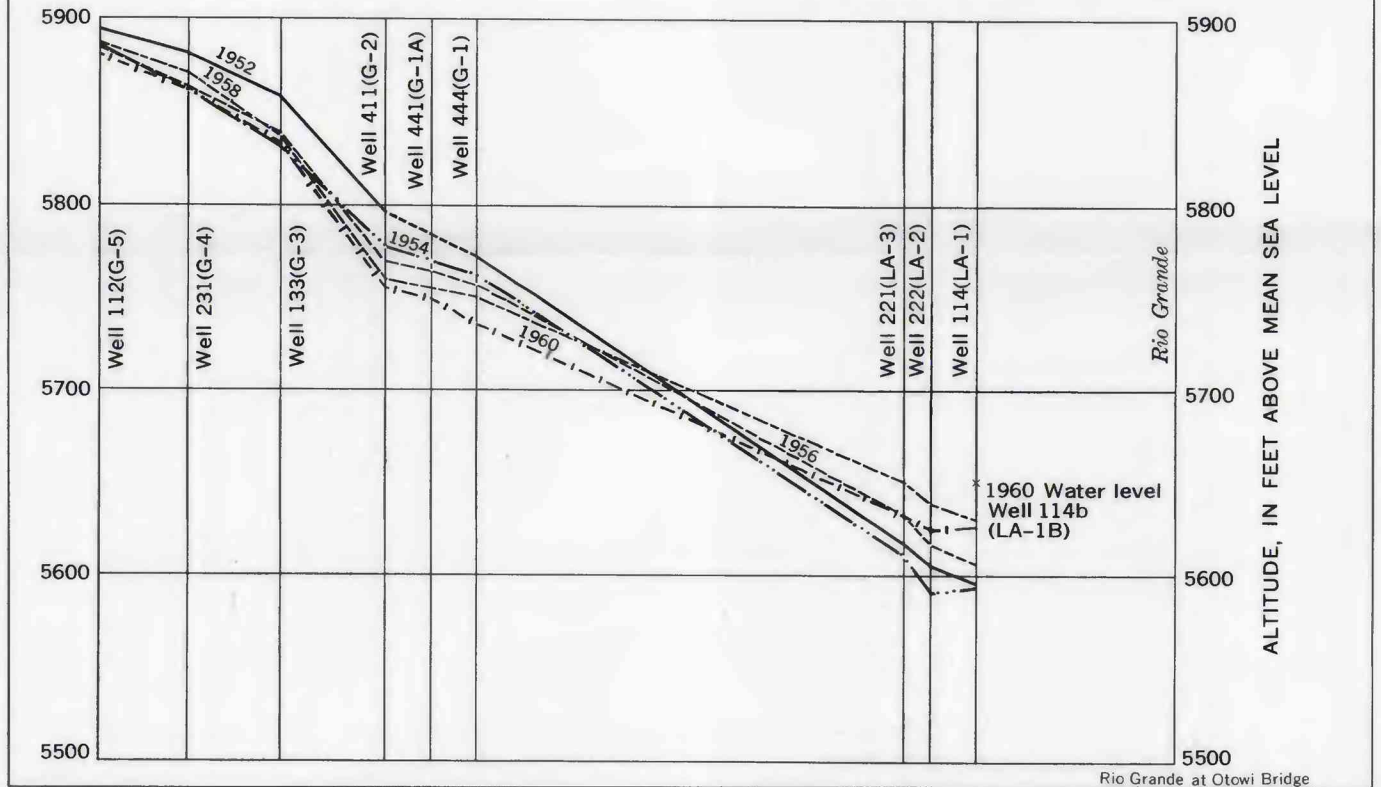
PROFILES OF THE PIEZOMETRIC SURFACE IN THE MAIN AQUIFER FOR SELECTED YEARS ALONG A LINE BETWEEN WELL 19.7.5.112(G-5) AND WELL 19.7.13.114(LA-1) NEAR LOS ALAMOS, NEW MEXICO
