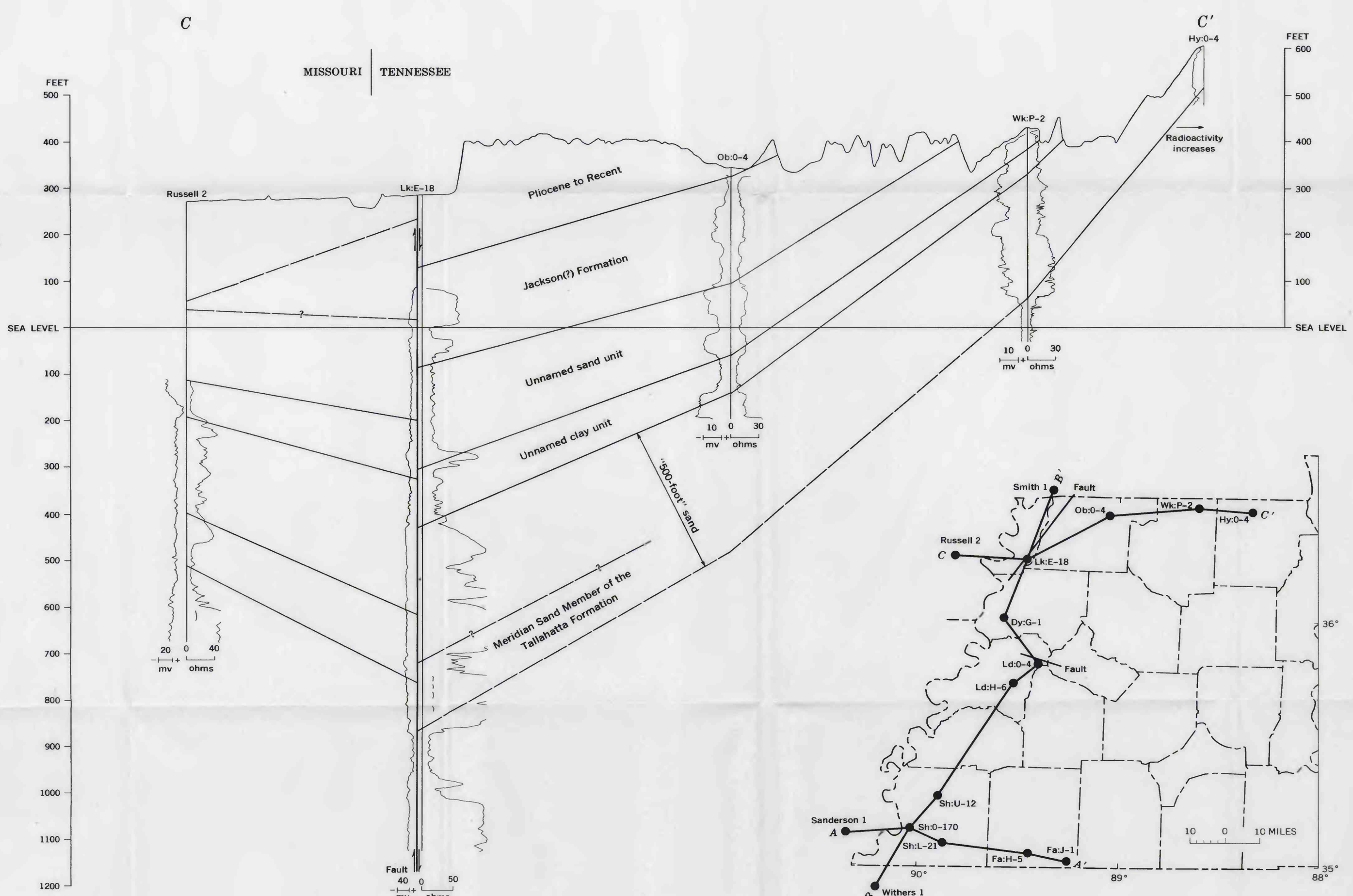
SECTION C-C' FROM PEMISCOT COUNTY, MO., TO HENRY COUNTY, TENN.
