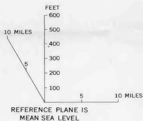
FENCE DIAGRAM AND ISOPACH MAP OF THE "500-FOOT" SAND IN WESTERN TENNESSEE
