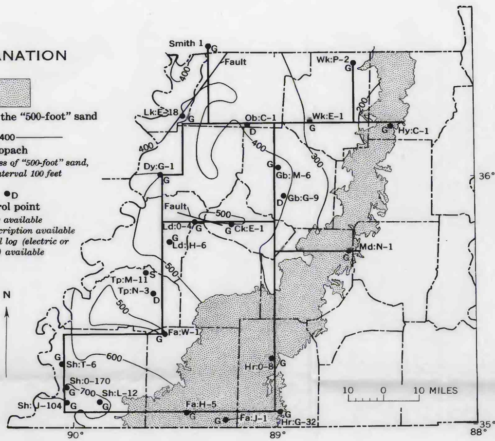
ISOPACH MAP OF "500-FOOT" SAND SHOWING SECTION LINES OF FENCE DIAGRAM
