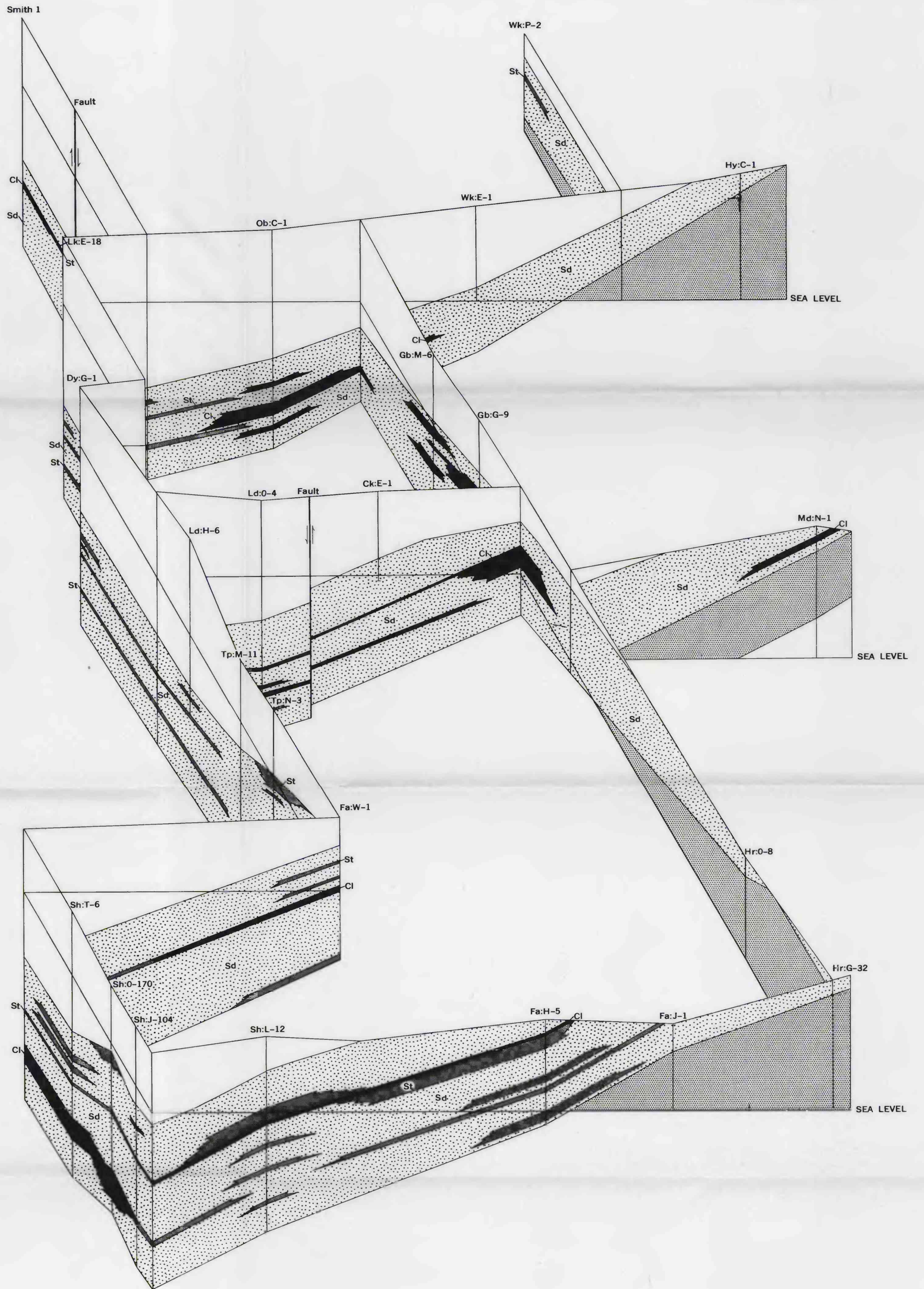
FENCE DIAGRAM AND ISOPACH MAP OF THE "500-FOOT" SAND IN WESTERN TENNESSEE
