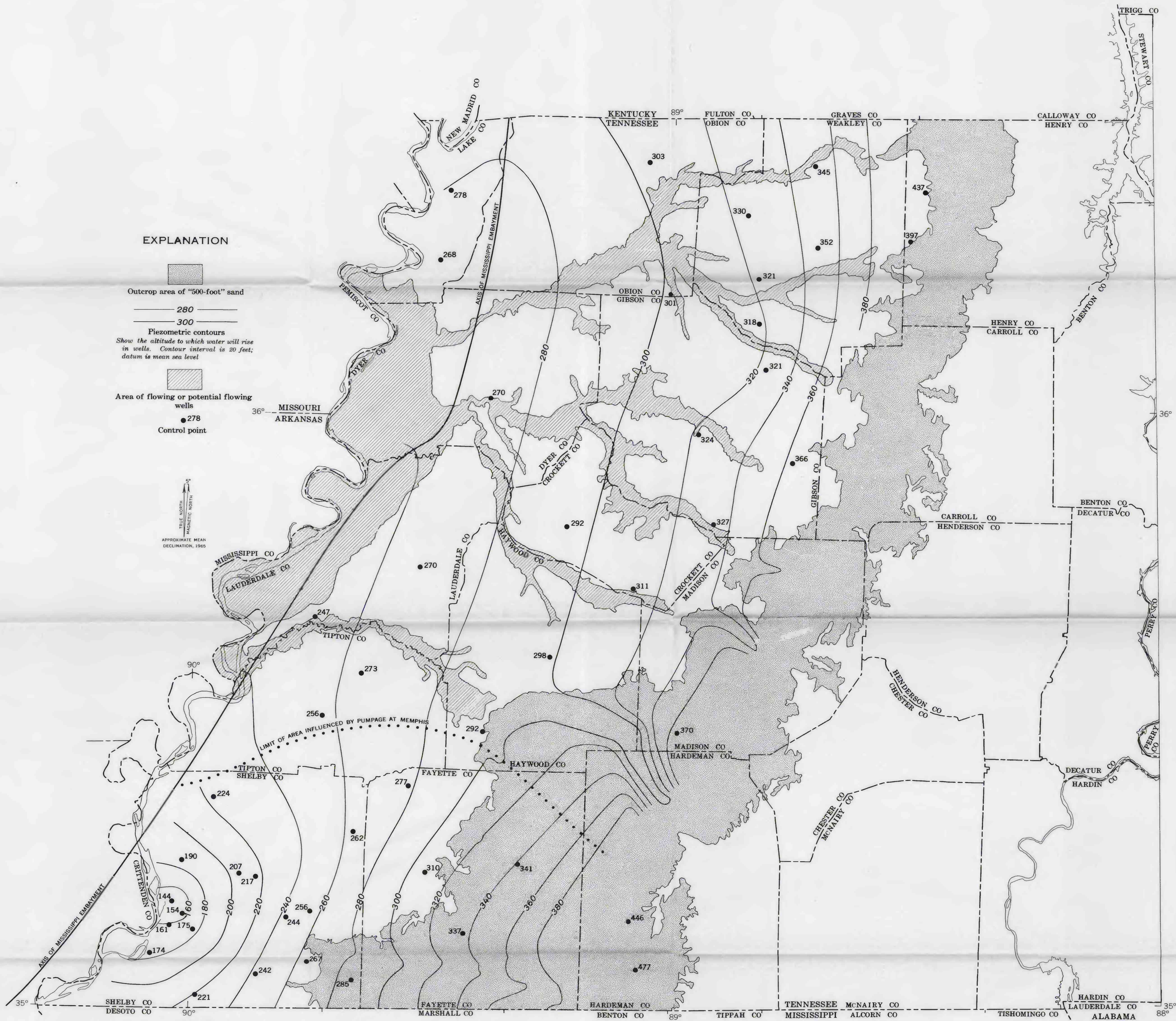
CONTOUR MAP OF THE PIEZOMETRIC SURFACE OF THE "500-FOOT" SAND IN WESTERN TENNESSEE, JANUARY 27-29, 1960
