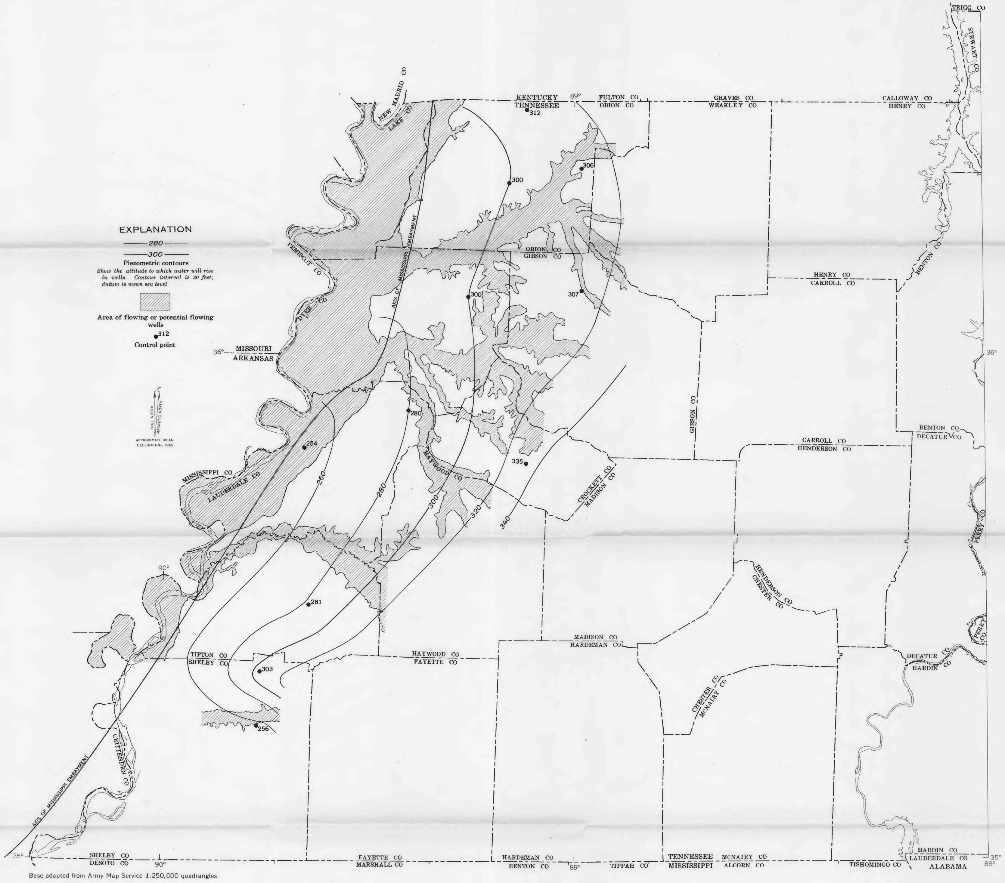
CONTOUR MAP OF THE PIEZOMETRIC SURFACE OF THE UNNAMED SAND UNIT IN WESTERN TENNESSEE, JANUARY 27-29, 1960
