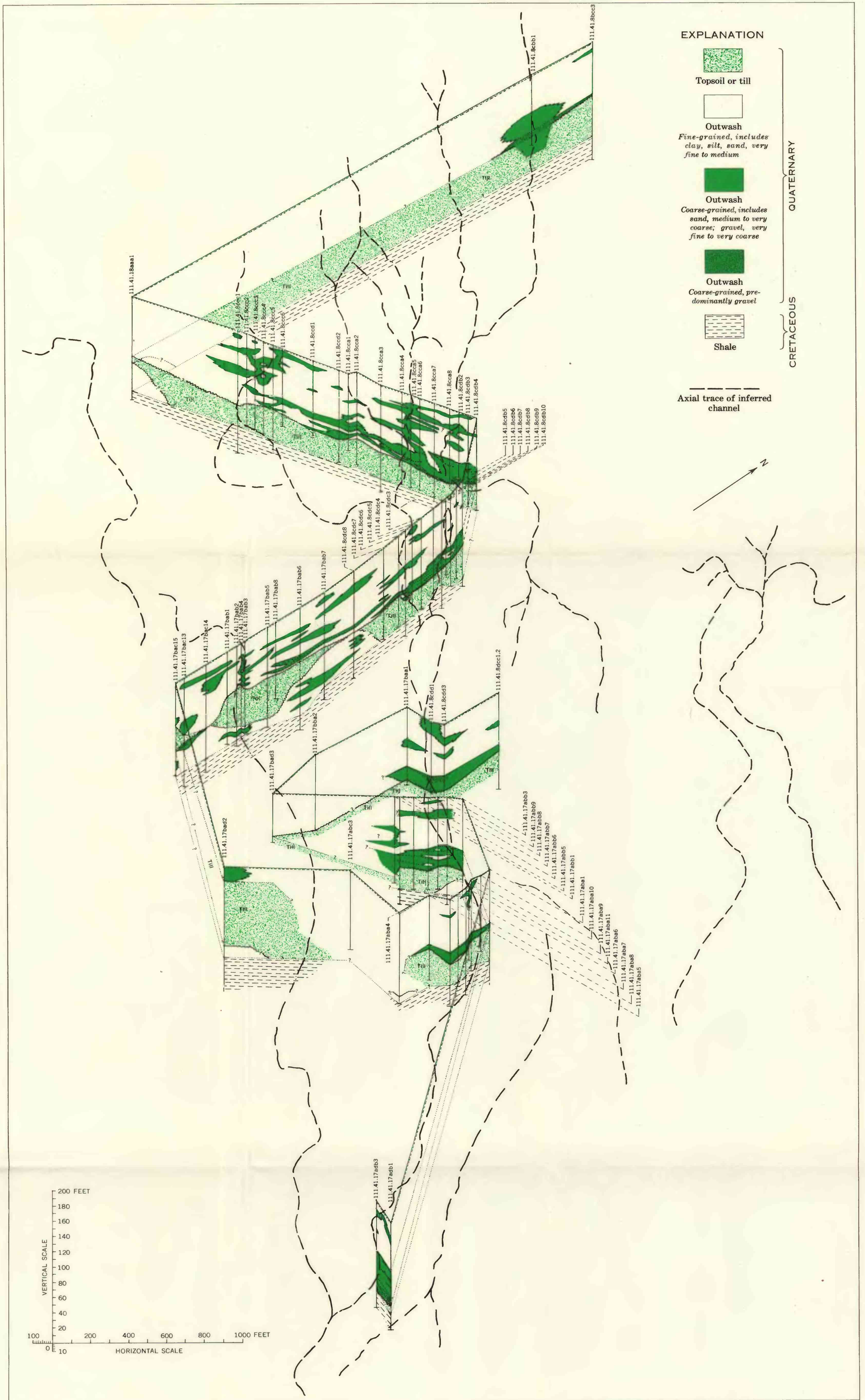
FENCE DIAGRAM SHOWING MELT-WATER AQUIFERS AND INFERRED AXIAL TRACES OF PROGLACIAL STREAM CHANNELS, MARSHALL AREA LYON COUNTY, MINNESOTA
