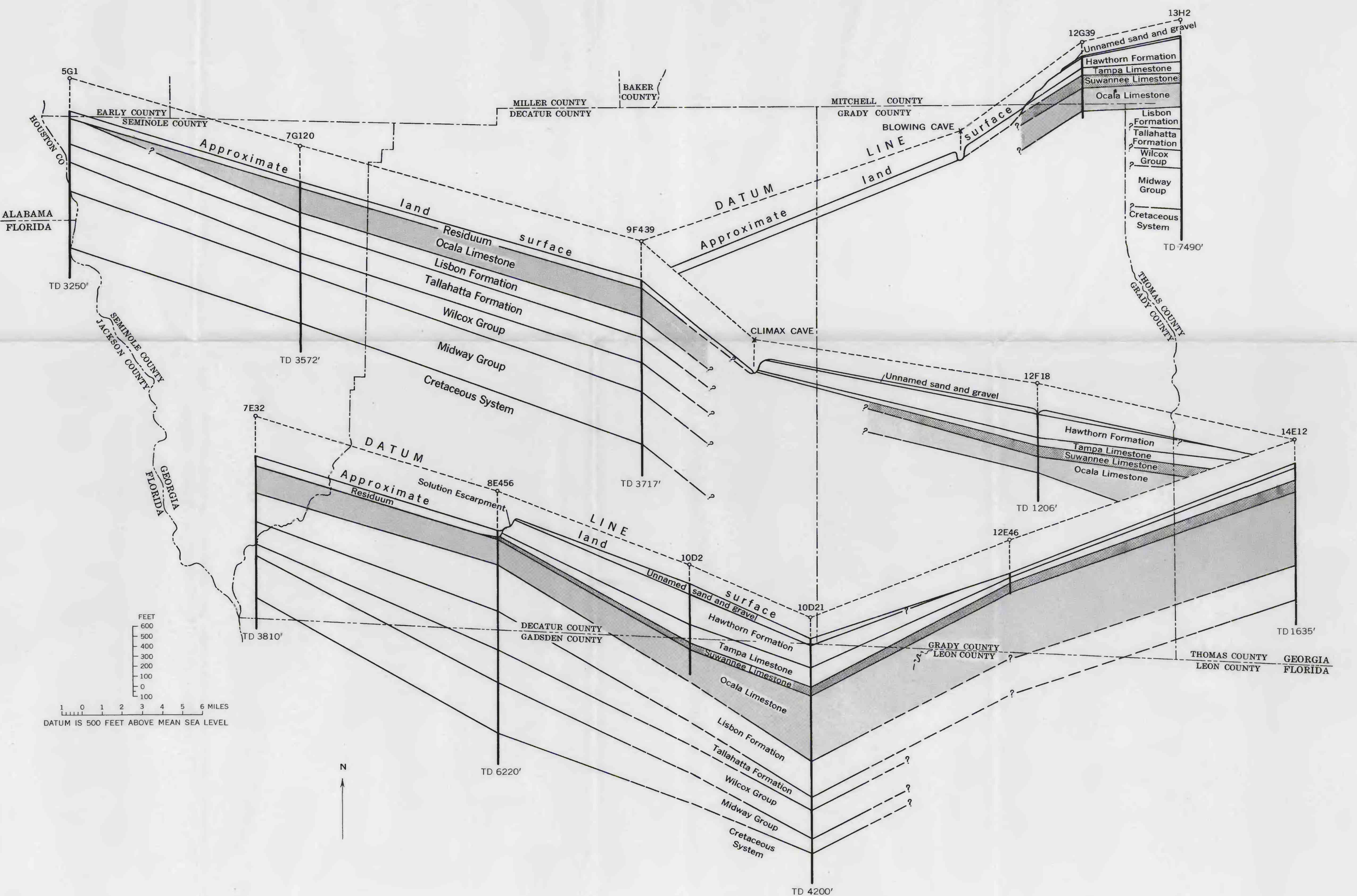
FENCE DIAGRAM
