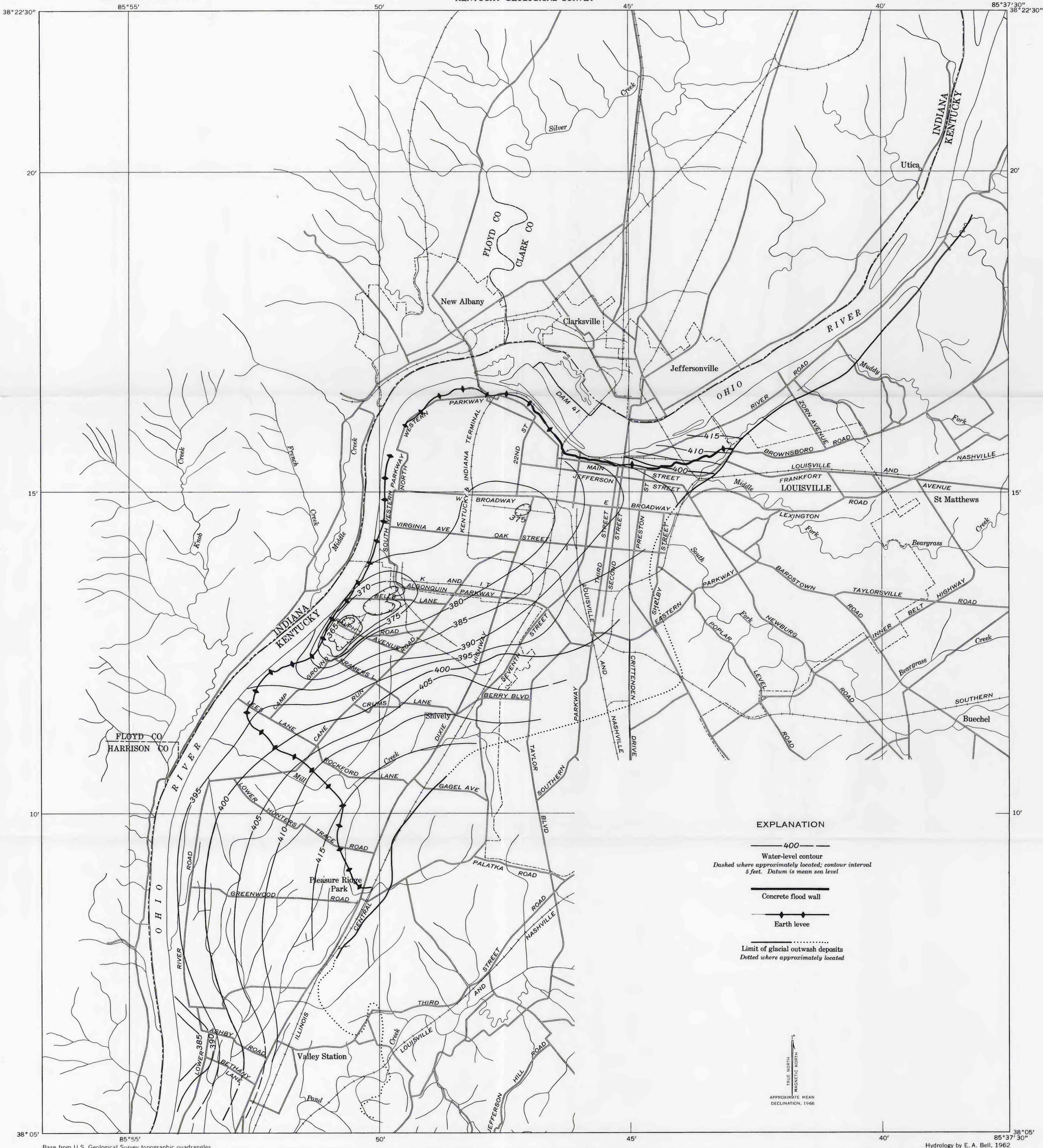
MAP SHOWING WATER-LEVEL CONTOURS BENEATH THE FLOOD PLAIN OF THE OHIO RIVER IN THE LOUISVILLE AREA, KENTUCKY, DECEMBER 1962
