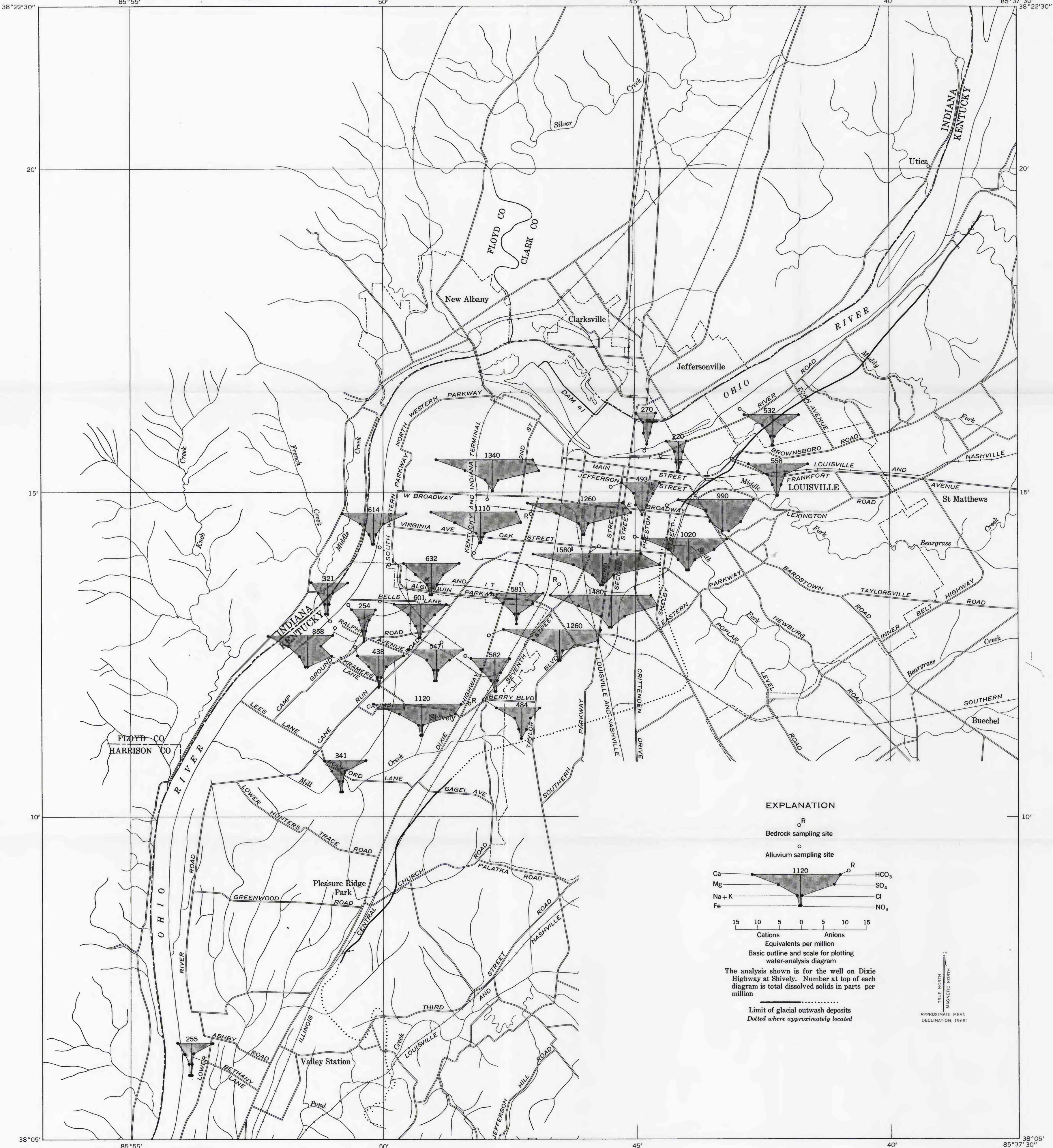
MAP SHOWING THE CHEMICAL CHARACTER OF GROUND WATER BENEATH THE FLOOD PLAIN OF THE OHIO RIVER IN THE LOUISVILLE AREA, KENTUCKY
