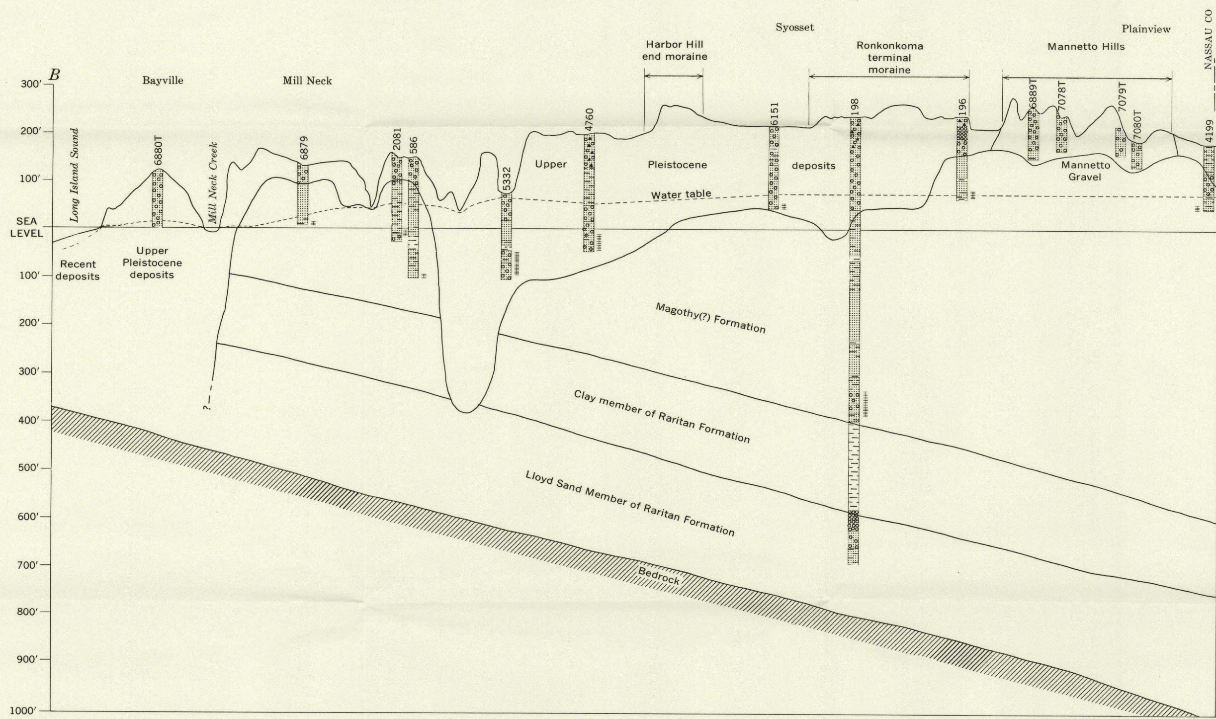
SECTION B-B', FROM LONG ISLAND SOUND NEAR BAYVILLE TO NASSAU COUNTY LINE AT PLAINVIEW
