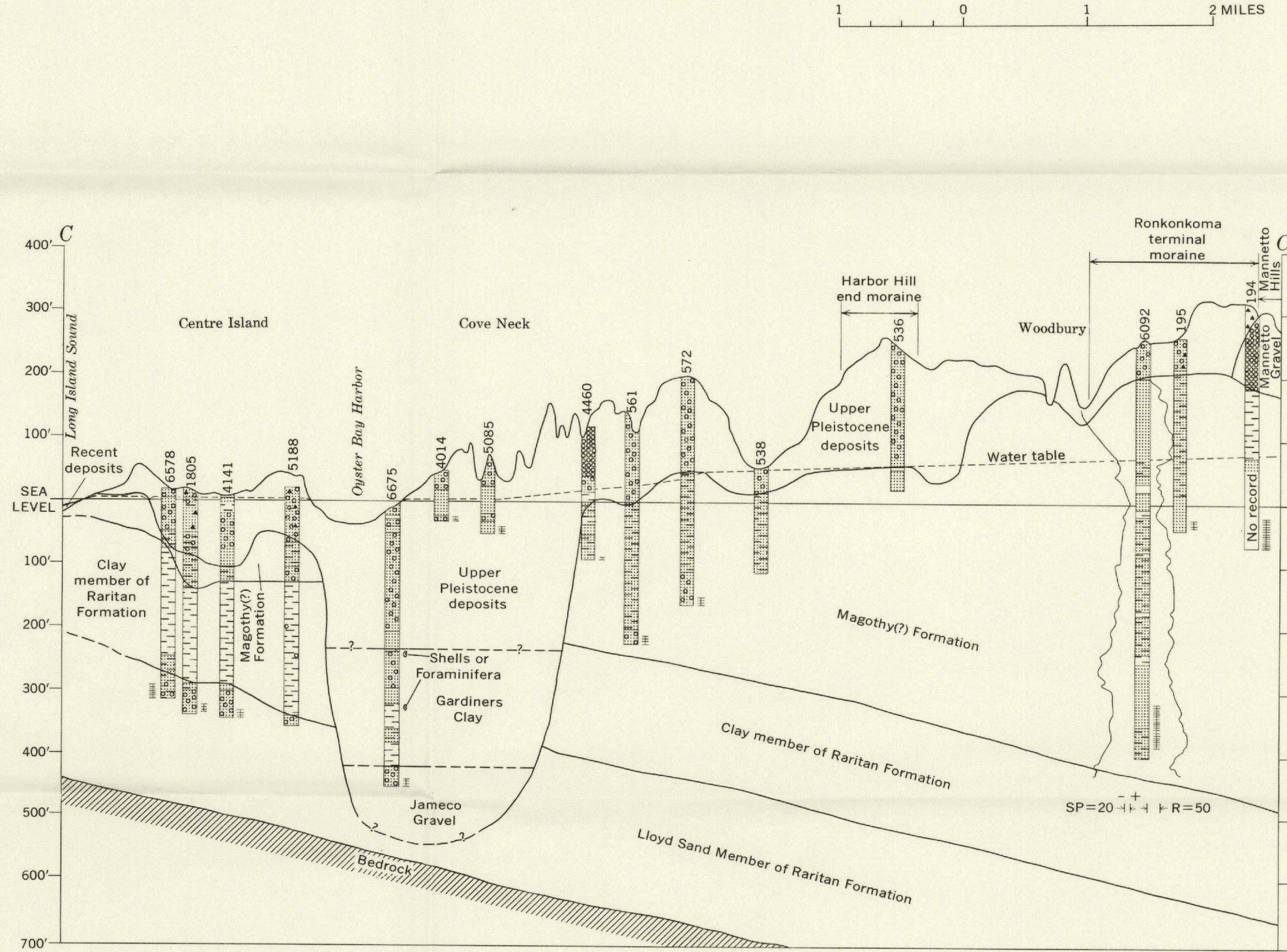
SECTION C-C', FROM LONG ISLAND SOUND NEAR CENTRE ISLAND TO NASSAU COUNTY LINE AT MANNETTO HILLS AT WOODBURY
