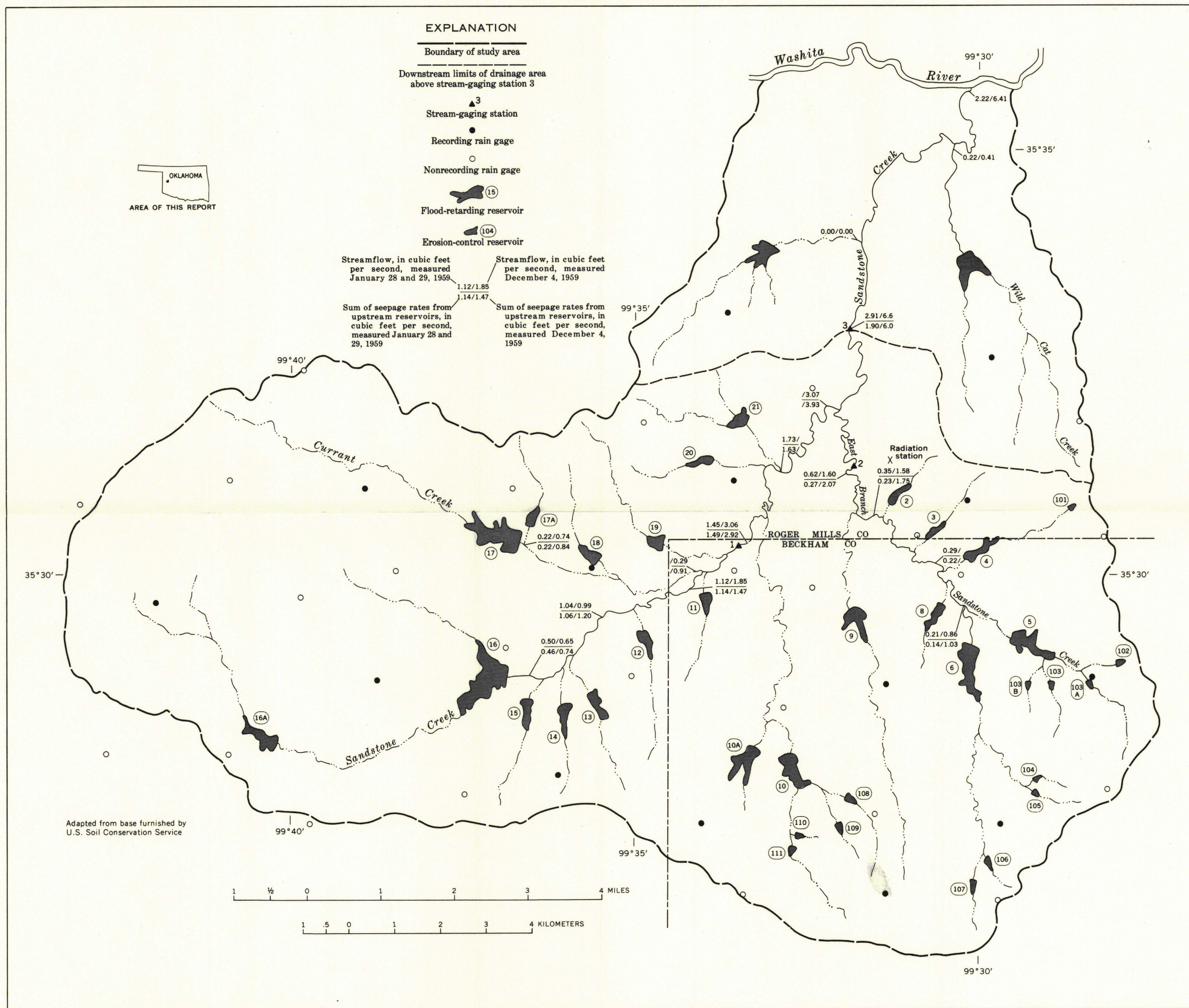
MAP OF SANDSTONE CREEK STUDY AREA, BECKHAM AND ROGER MILLS COUNTIES, WESTERN OKLAHOMA, SHOWING LOCATION OF RESERVOIRS, DATA STATIONS, AND RESERVOIR-SEEPAGE MEASUREMENTS MADE IN JANUARY AND DECEMBER 1959
