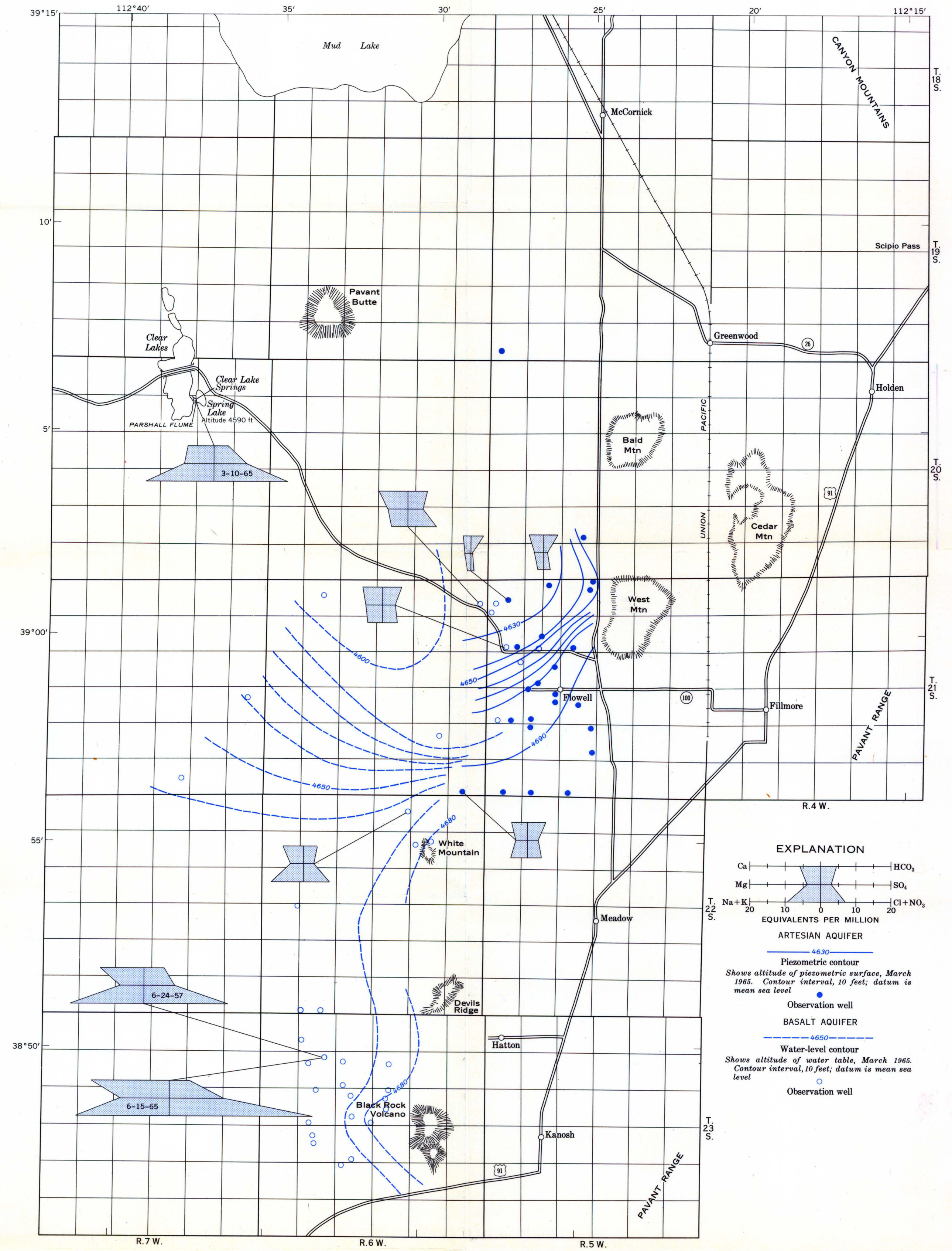
WATER-LEVELS AND QUALITY OF WATER IN THE BASALT AND THE ARTESIAN AQUIFERS
