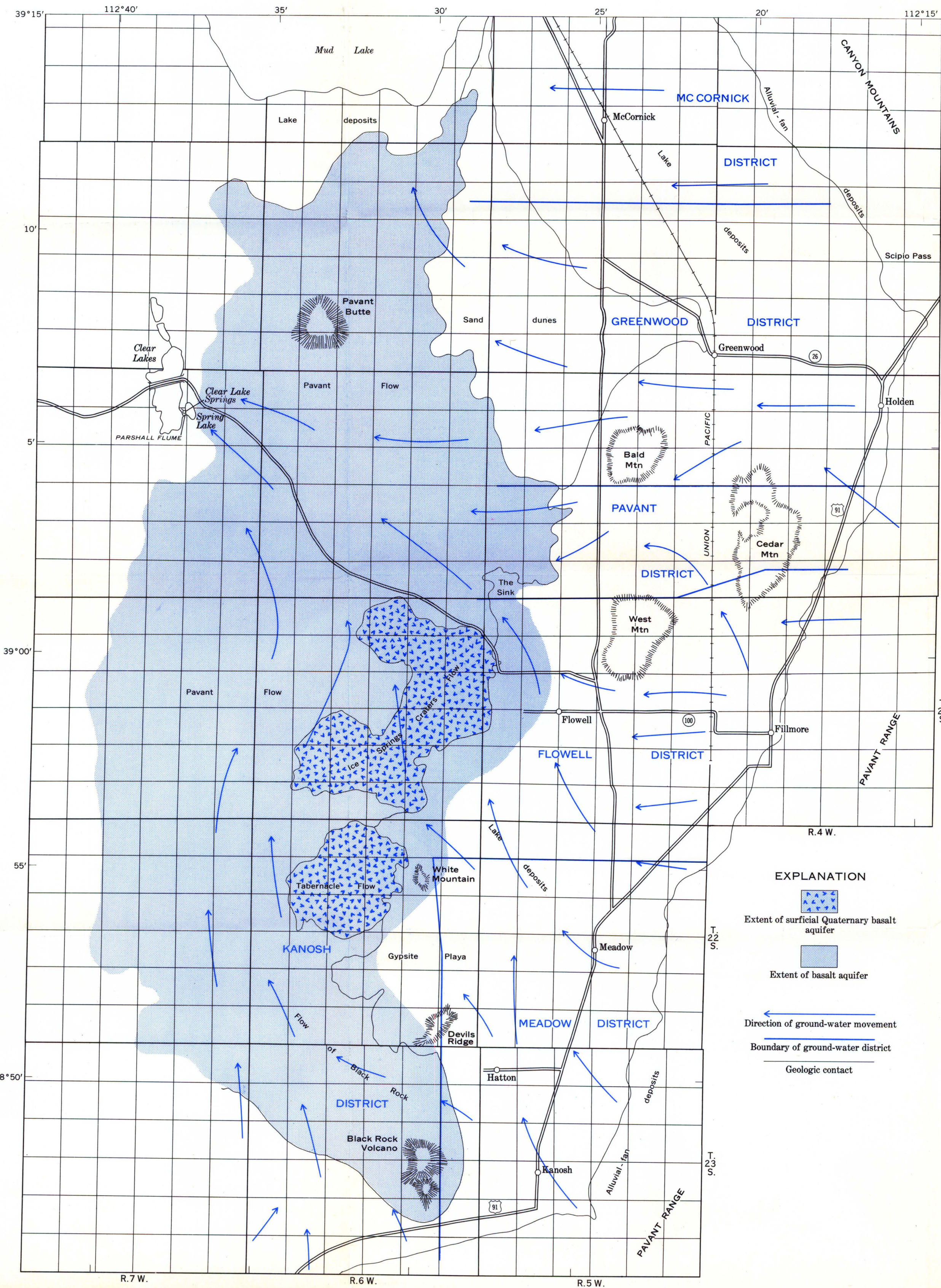
GENERALIZED GEOLOGY AND DIRECTION OF GROUND-WATER MOVEMENT
