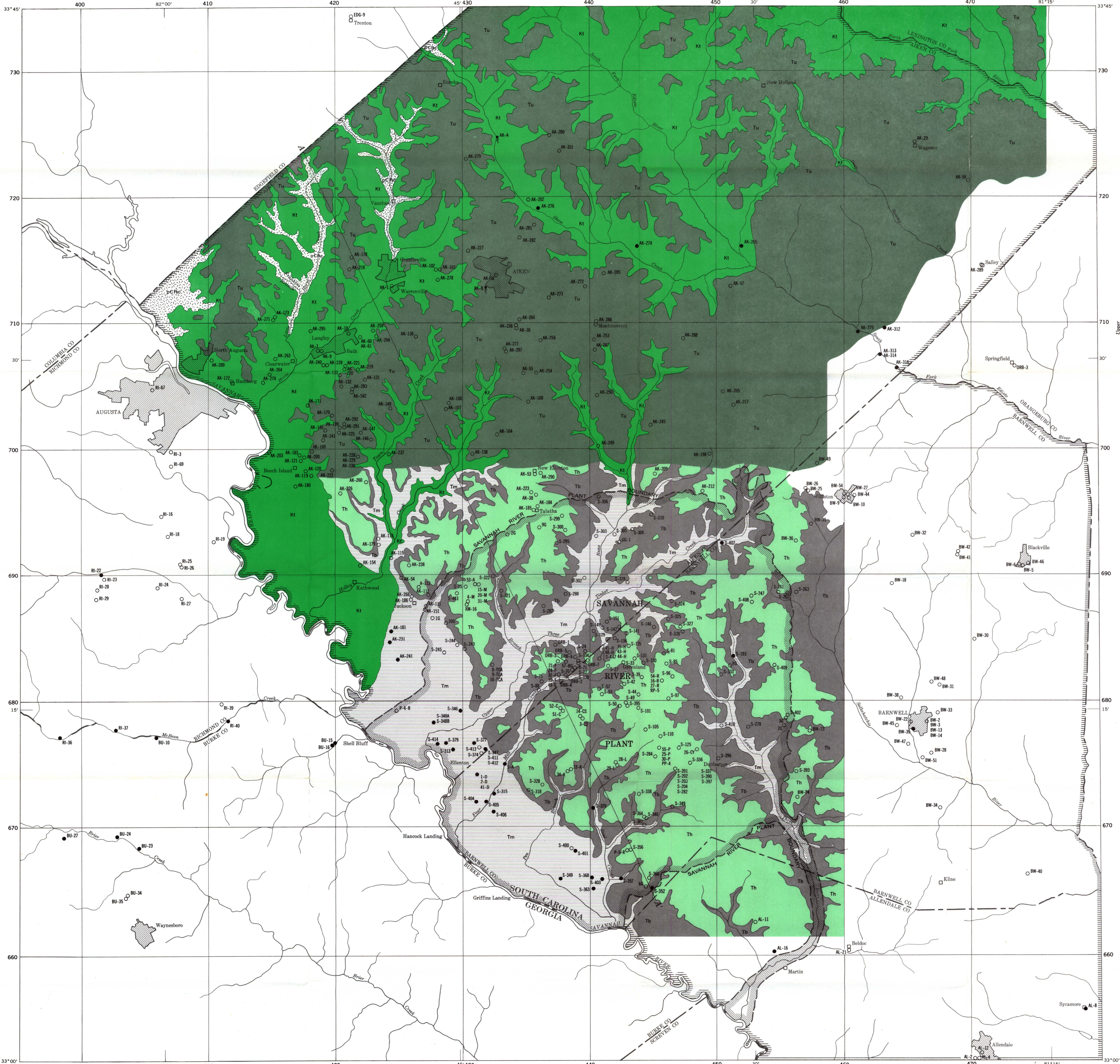
GEOLOGIC MAP SHOWING LOCATION OF WELLS AND SPRINGS IN THE SAVANNAH RIVER PLANT AREA, SOUTH CAROLINA
