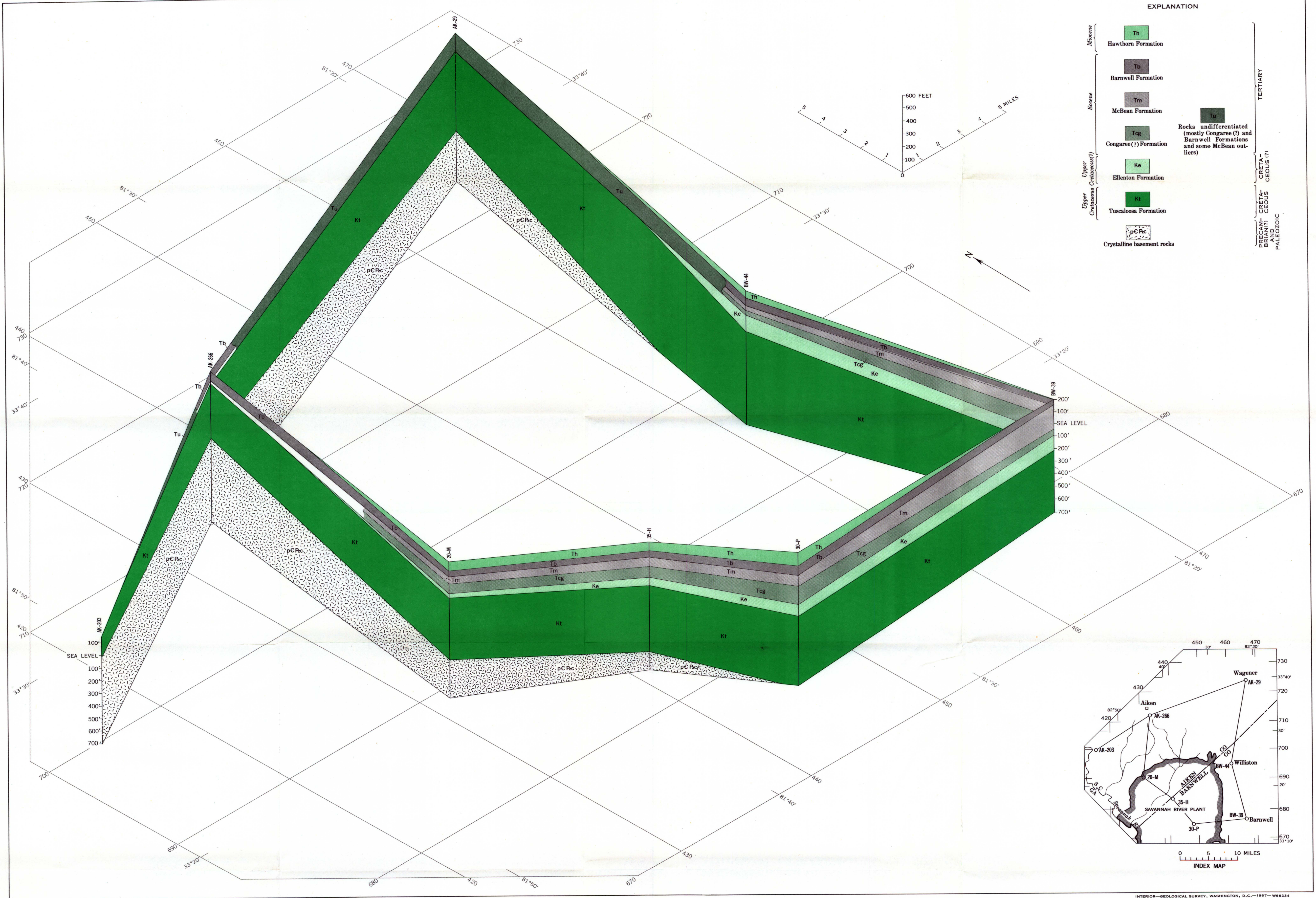
FENCE DIAGRAM SHOWING SUBSURFACE GEOLOGY IN SAVANNAH RIVER PLANT AREA, SOUTH CAROLINA
