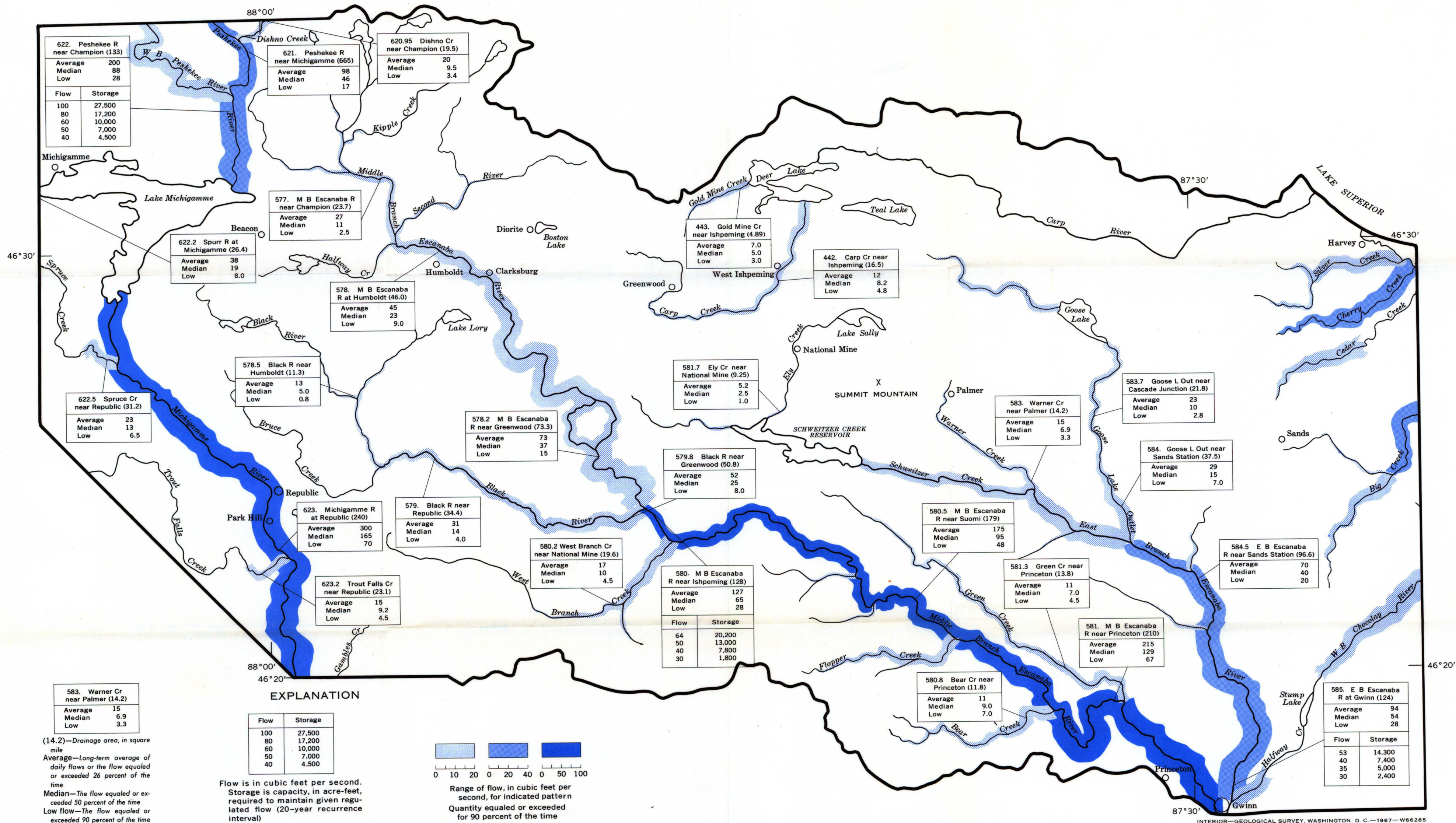
MAP SHOWING THE AVAILABILITY OF STREAMFLOW IN THE MARQUETTE IRON RANGE AREA, MICHIGAN
