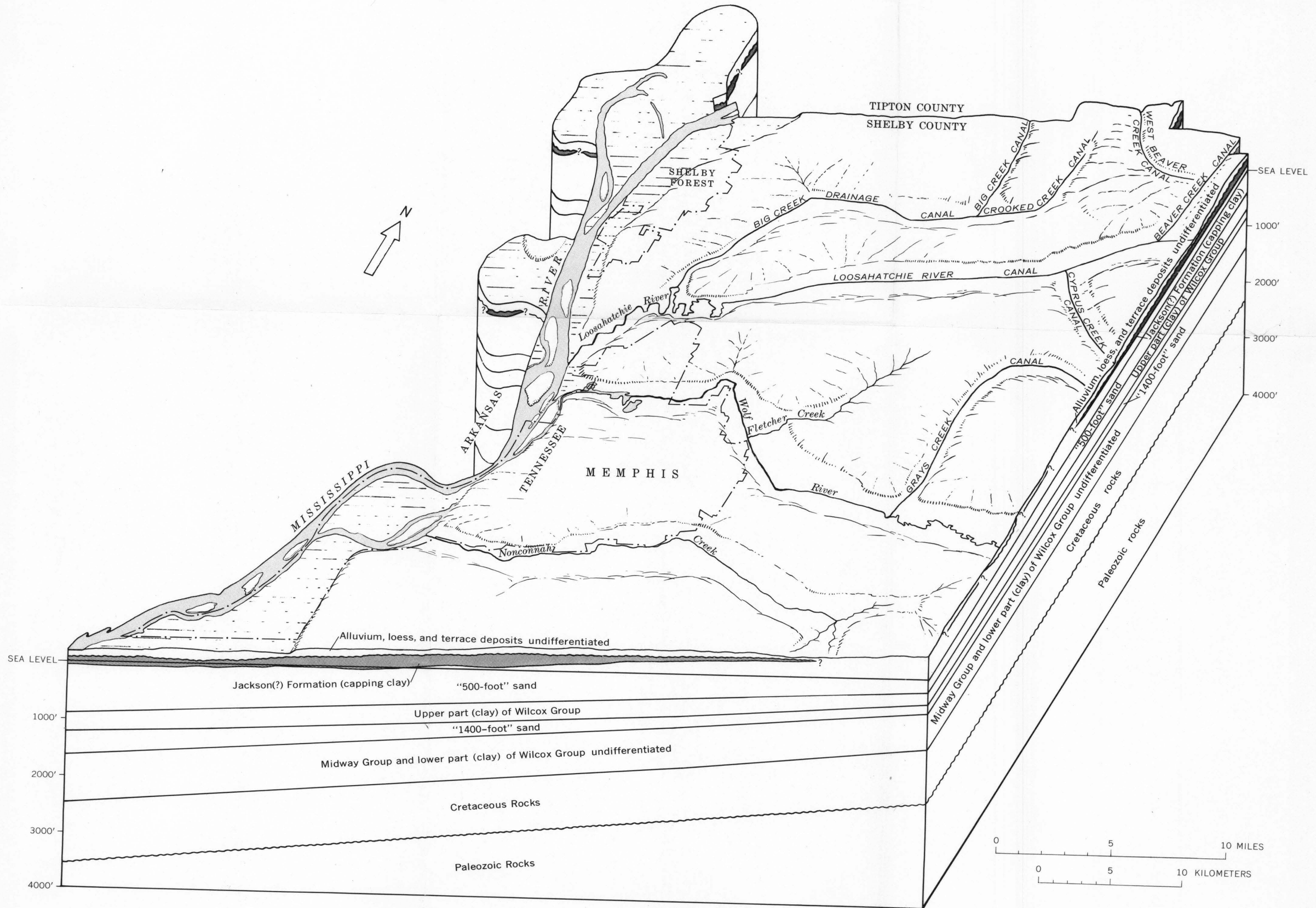
BLOCK DIAGRAM SHOWING PHYSIOGRAPHIC AND GEOLOGIC FEATURES OF THE MEMPHIS AREA, TENNESSEE
