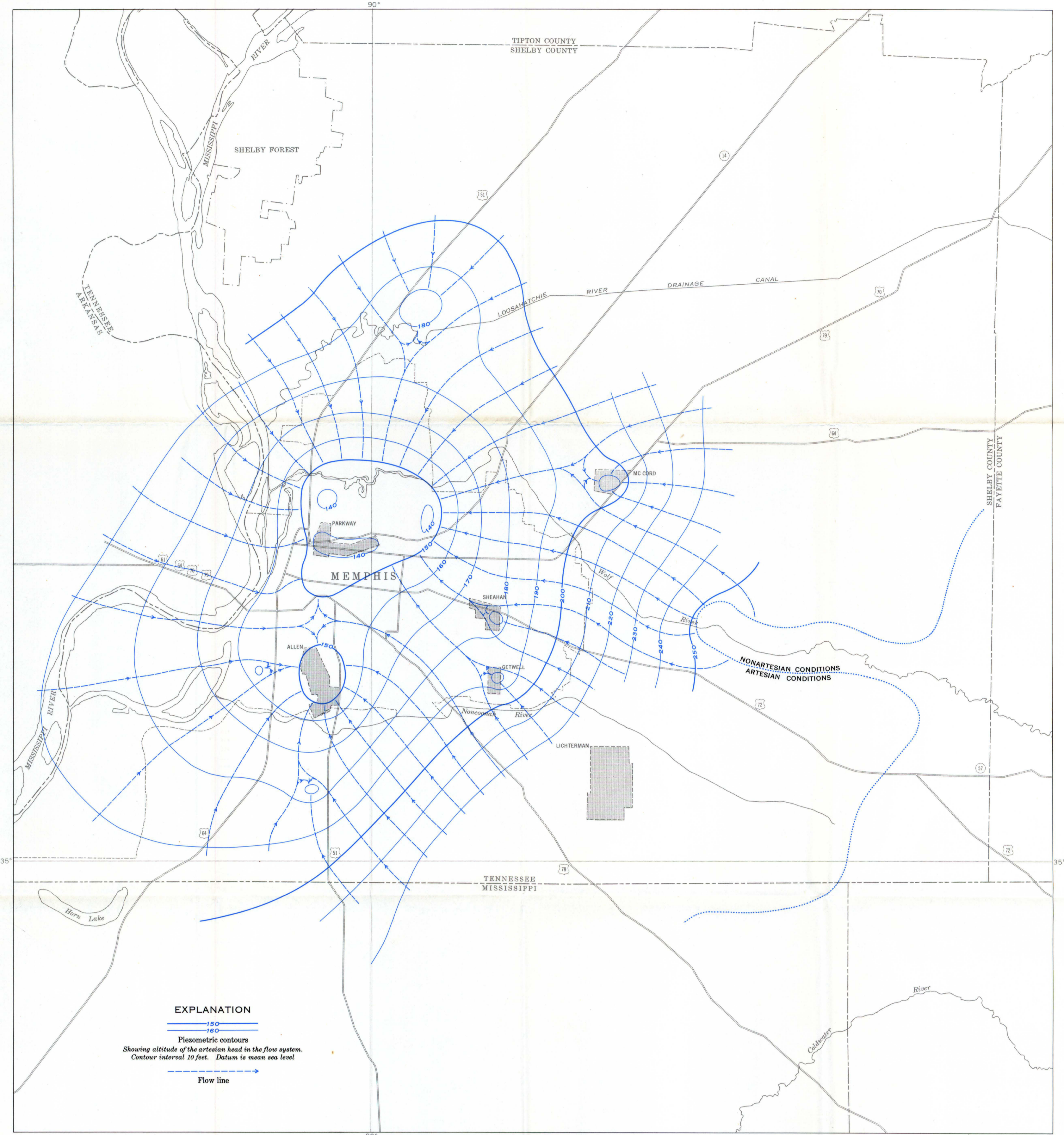
B. FLOW NET IN APRIL 1964
