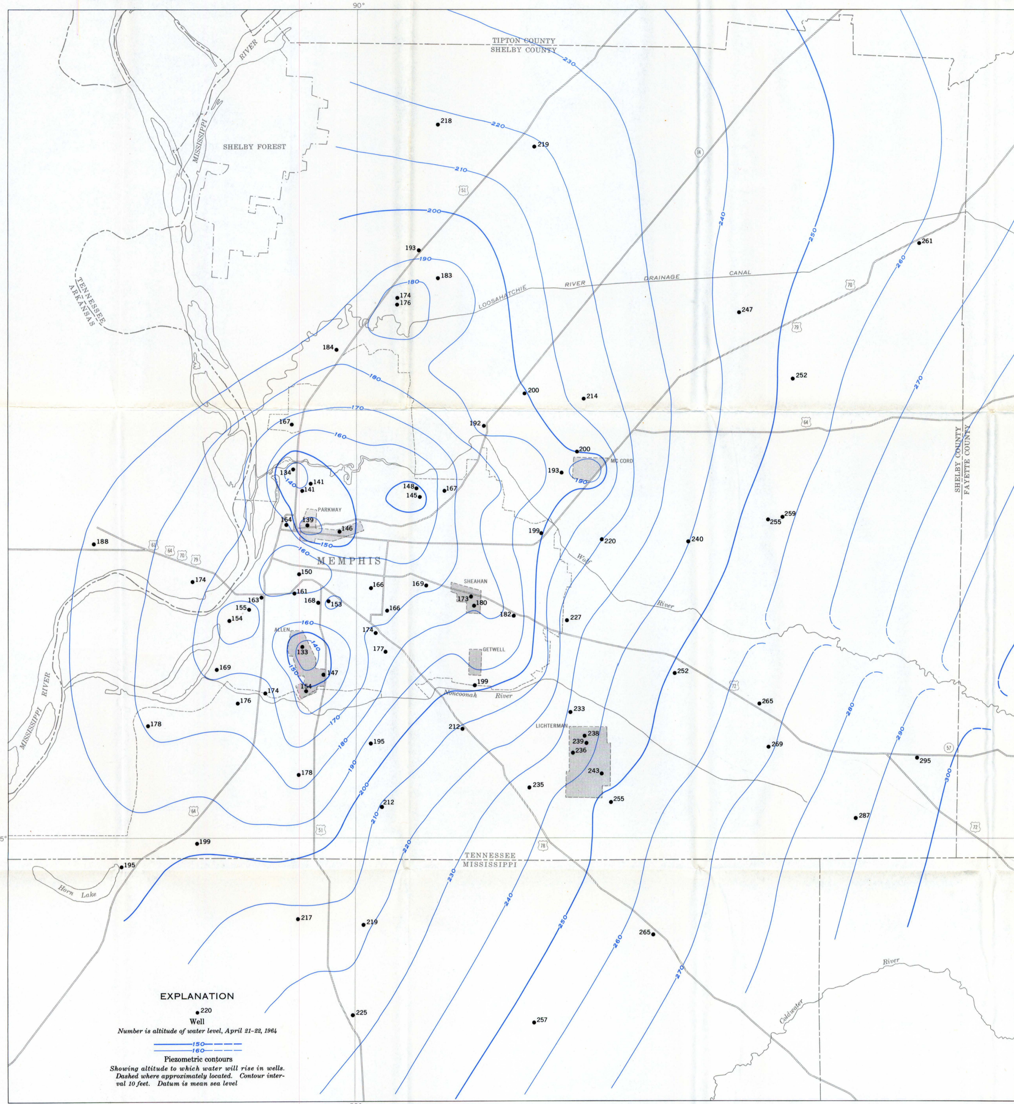
A. PIEZOMETRIC SURFACE IN APRIL 1964
