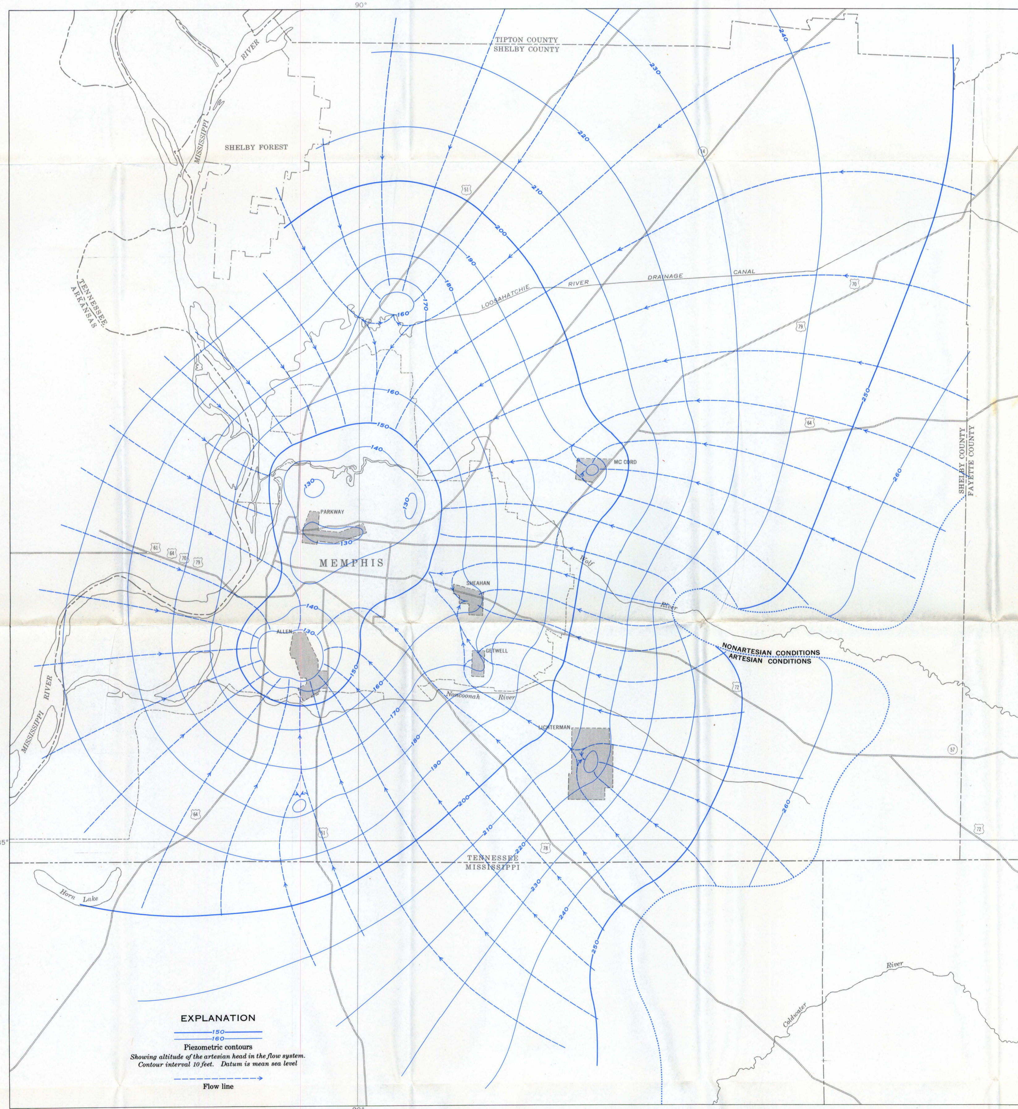
C. PREDICTED FLOW NET IN 1975
