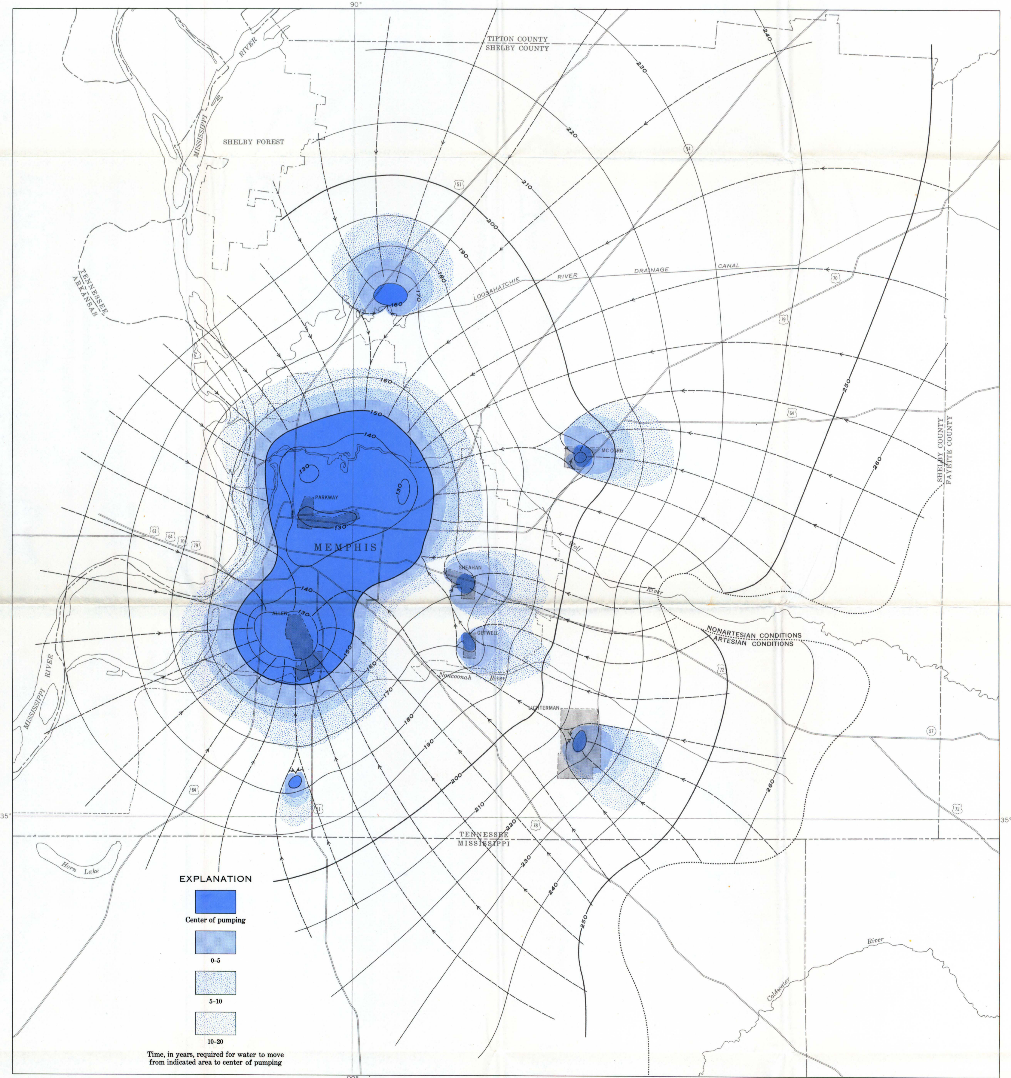
D. TIME REQUIRED FOR WATER TO MOVE FROM INDICATED AREAS TO CENTERS OF HEAVY PUMPING (REFERENCED TO ESTIMATED PUMPING IN 1975)
