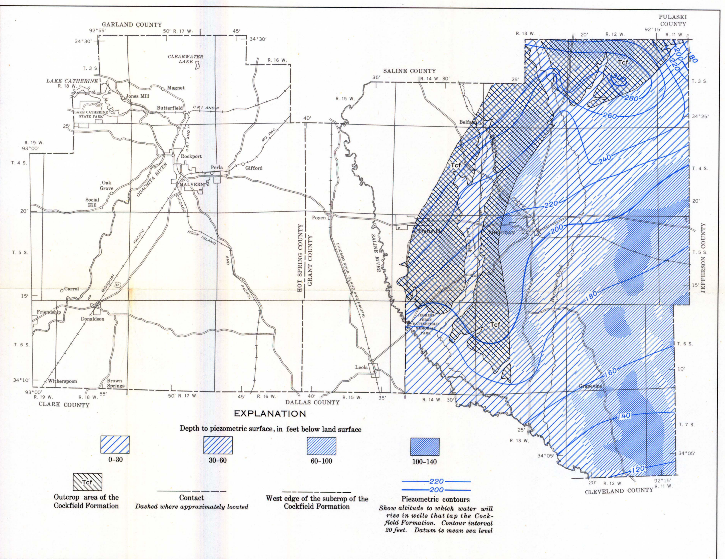
OUTCROP AREA AND DEPTH TO AND ALTITUDE OF THE PIEZOMETRIC SURFACE IN THE COCKFIELD FORMATION
