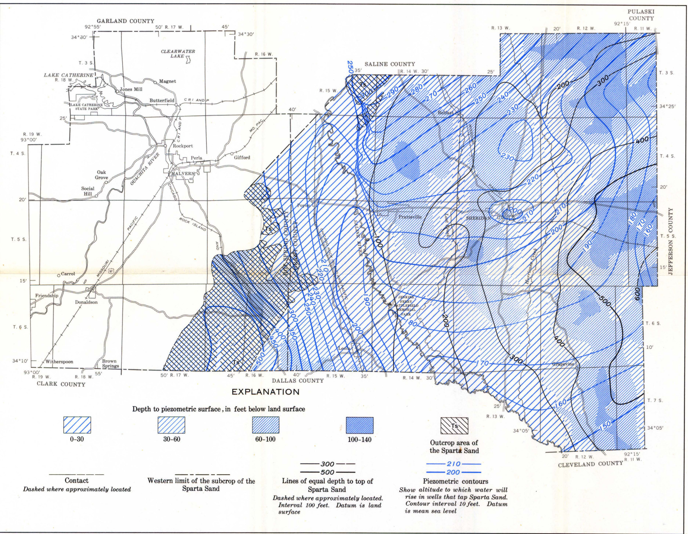
OUTCROP AREA, DEPTH TO TOP OF SPARTA SAND, AND DEPTH TO AND ALTITUDE OF THE PIEZOMETRIC SURFACE
