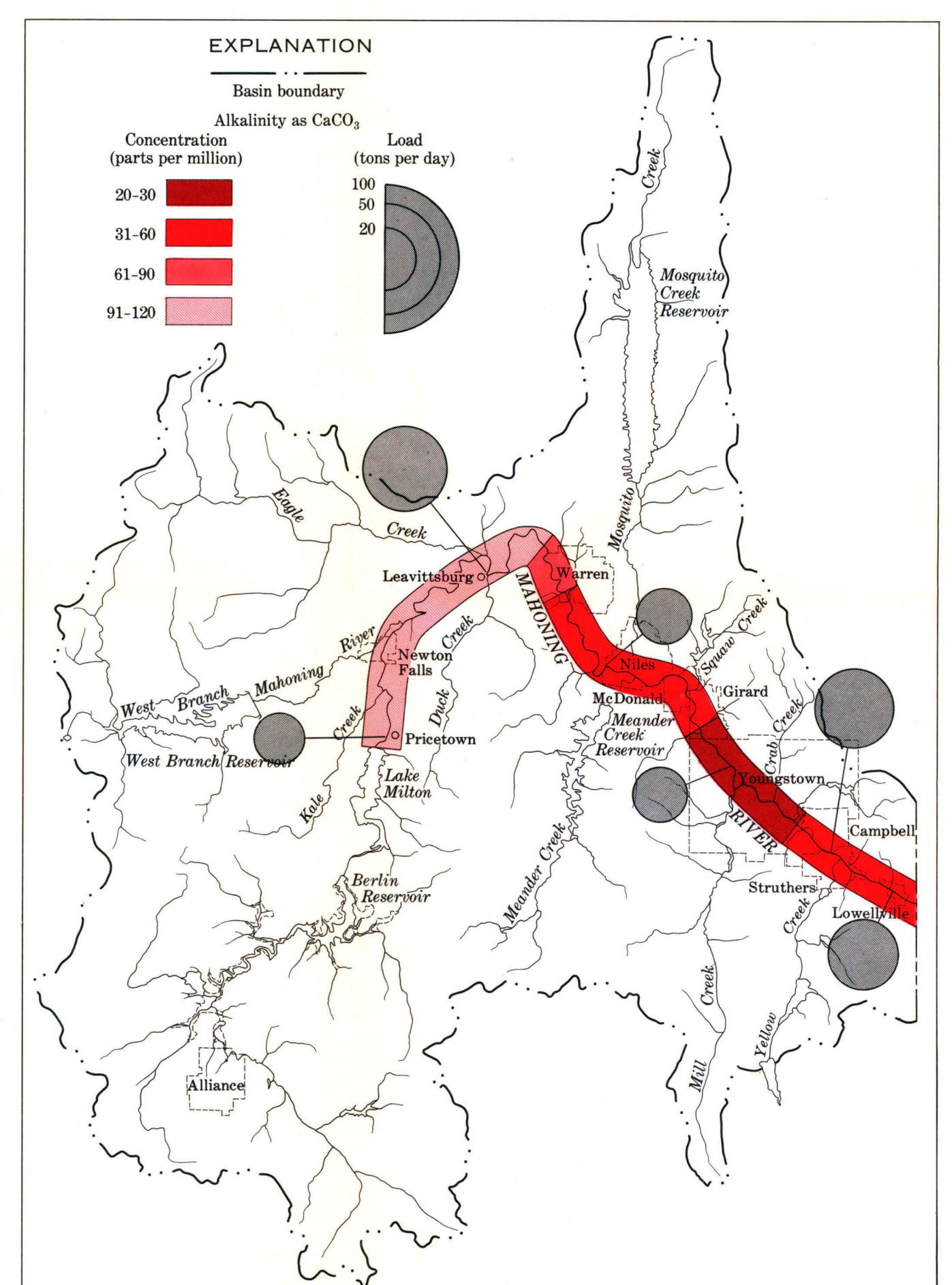
ALKALINITY (AS CaCO 3 ) CONCENTRATION AND LOAD DURING LOW STREAMFLOW Discharge equalled or exceeded 90 percent of the time
