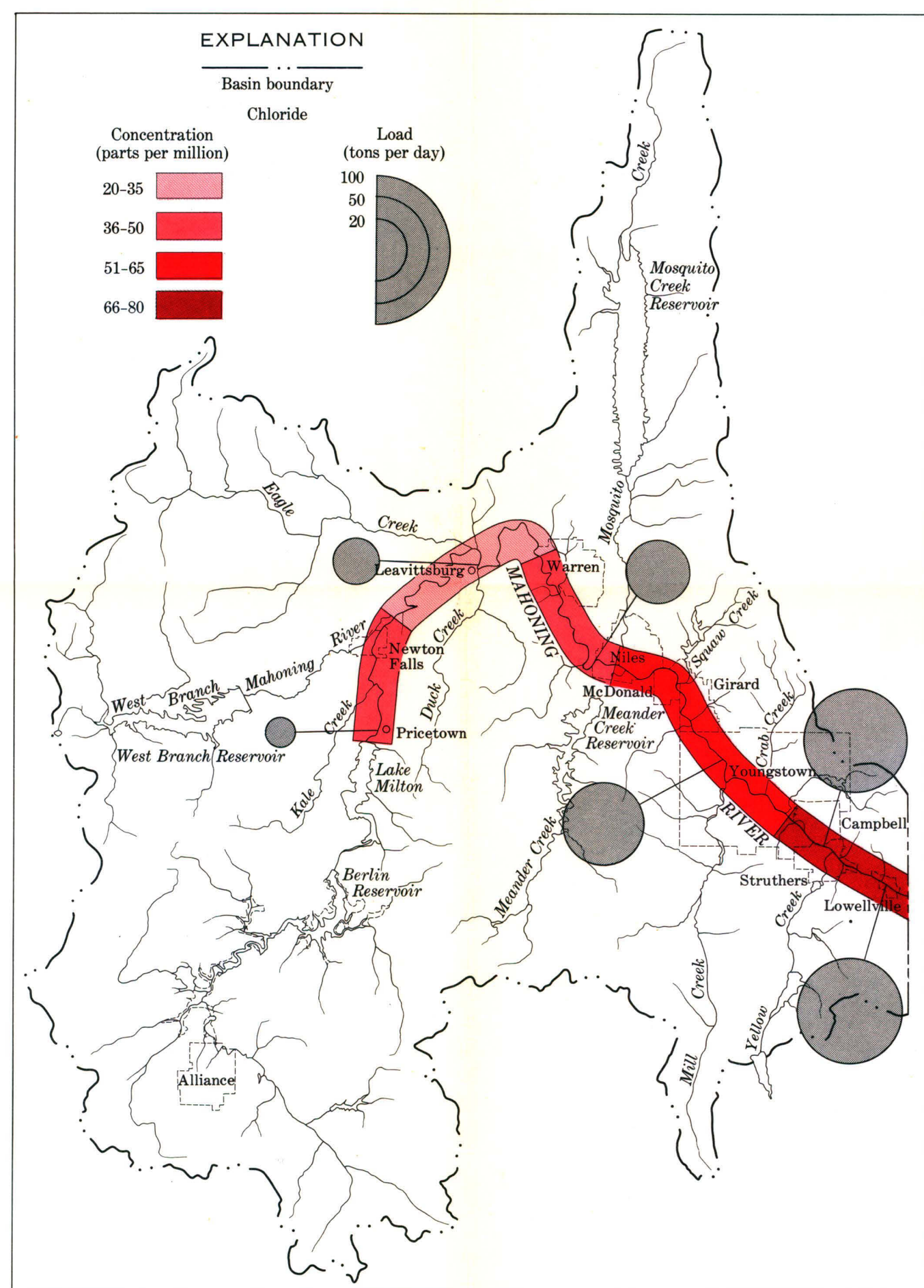
CHLORIDE CONCENTRATION AND LOAD DURING LOW STREAMFLOW Discharge equalled or exceeded 90 percent of the time
