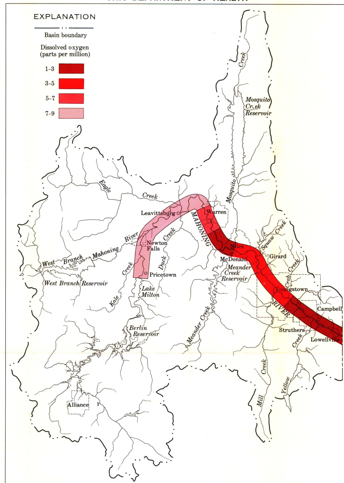
DISSOLVED-OXYGEN CONCENTRATION—For 10 percent of the time the dissolved-oxygen concentration was equal to or less than that shown
