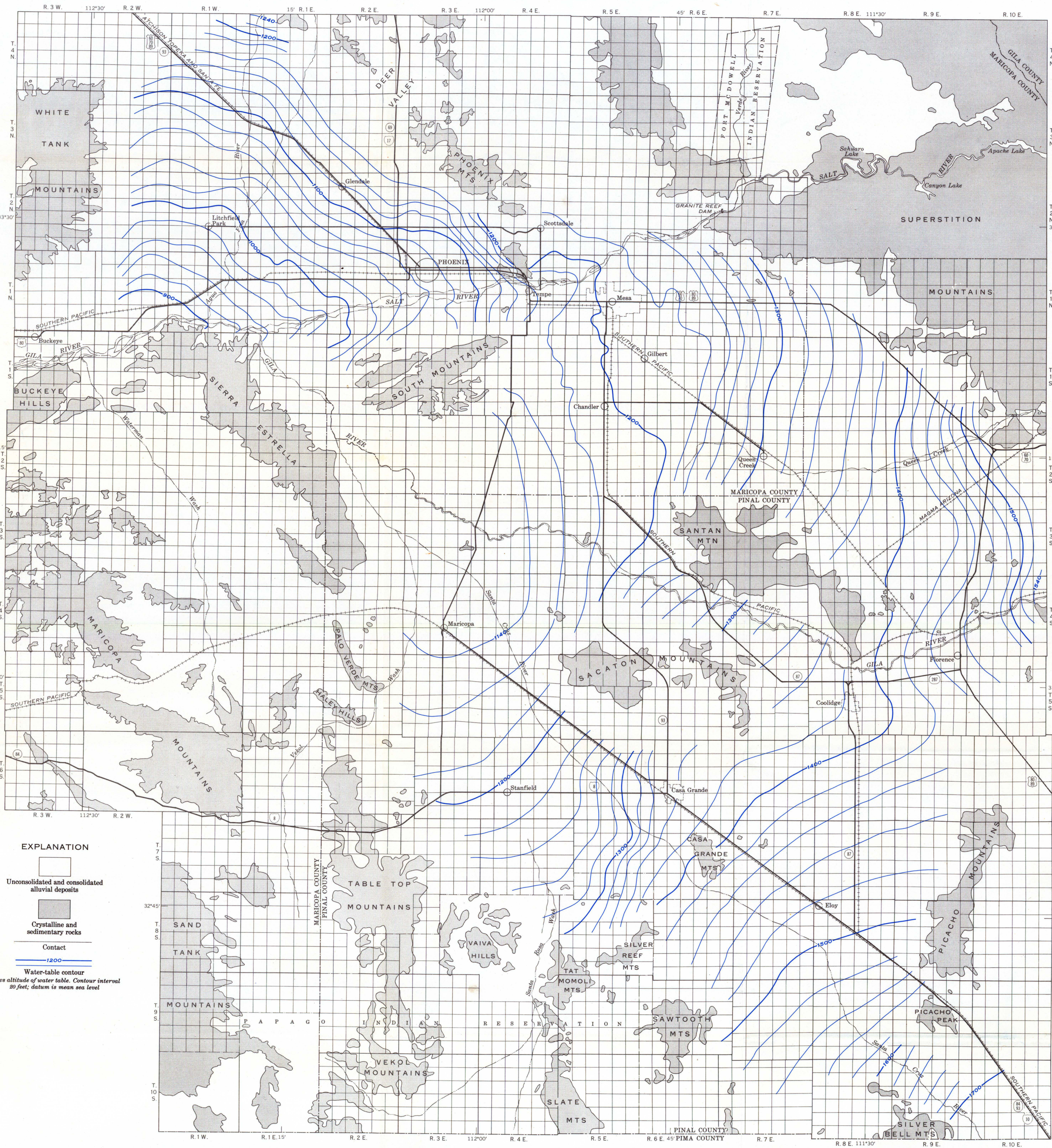
ALTITUDE OF THE WATER TABLE, SPRING 1923
