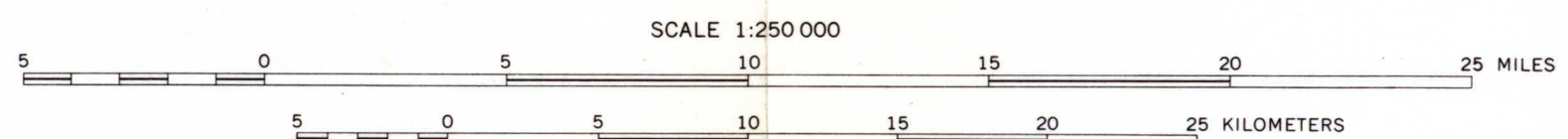
MAPS SHOWING PREDICTED DEPTHS TO WATER IN CENTRAL ARIZONA
