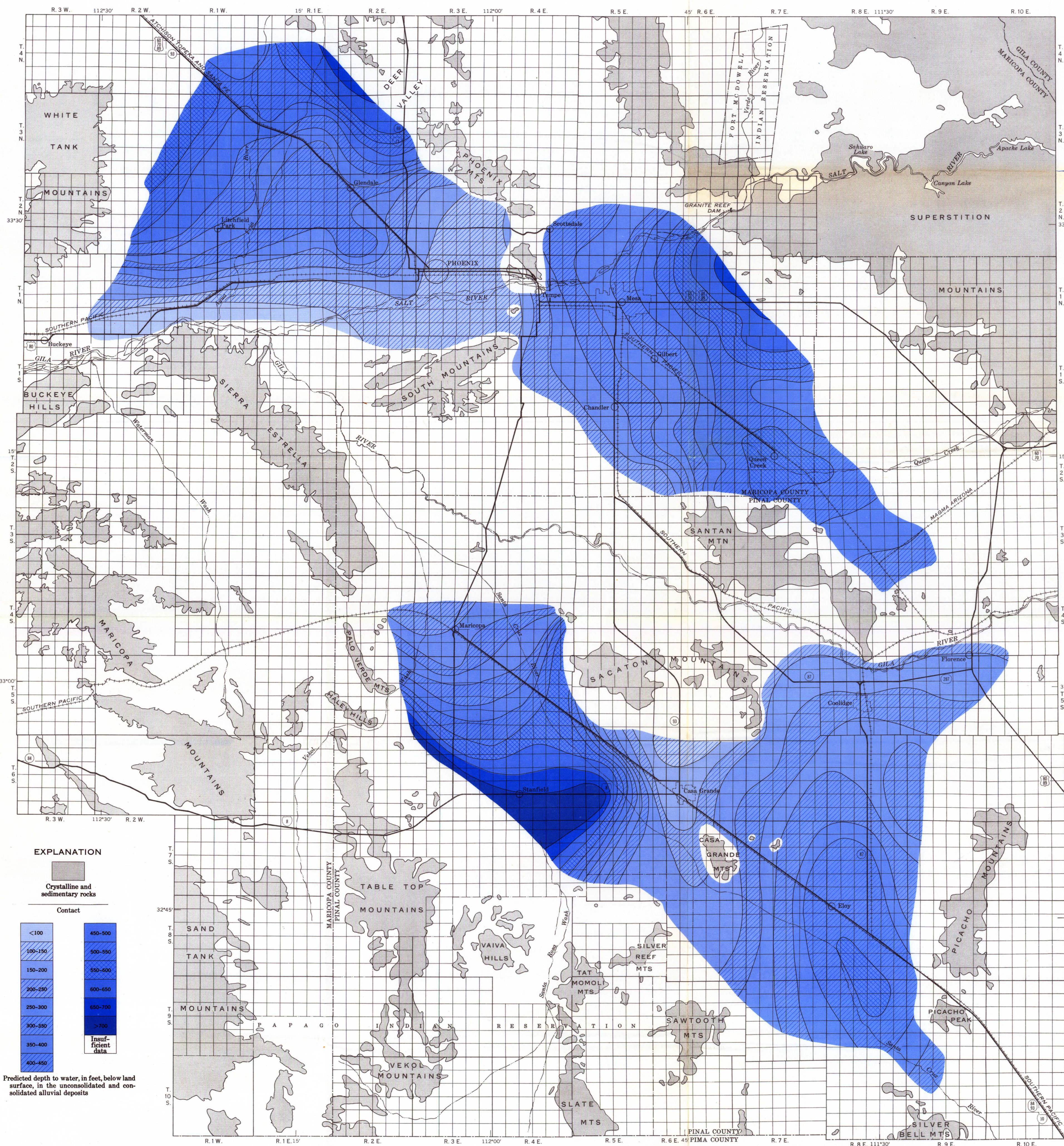
MAPS SHOWING PREDICTED DEPTHS TO WATER IN CENTRAL ARIZONA
