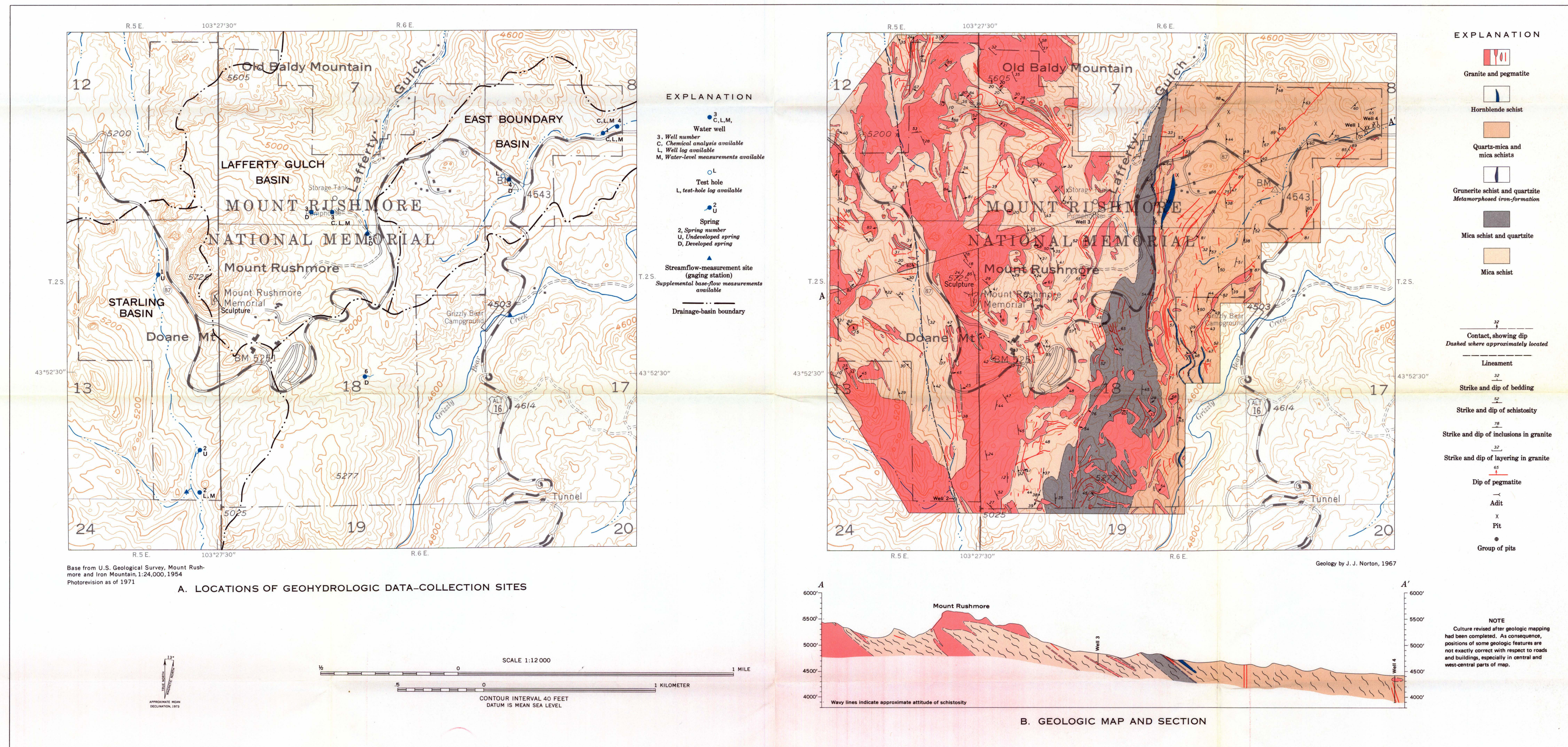
GEOHYDROLOGIC MAPS OF THE MOUNT RUSHMORE NATIONAL MEMORIAL, SOUTH DAKOTA
