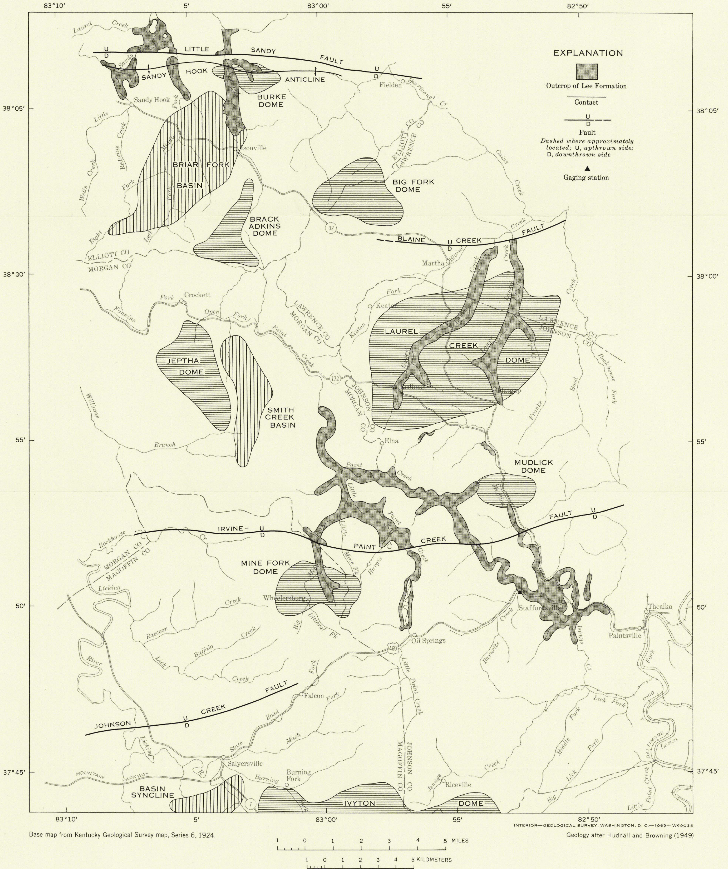
MAP SHOWING MAJOR STRUCTURAL FEATURES AND OUTCROP AREAS OF THE LEE FORMATION IN PARTS OF ELLIOTT, JOHNSON, LAWRENCE, MAGOFFIN, AND MORGAN COUNTIES, EASTERN COAL FIELD REGION, KENTUCKY
