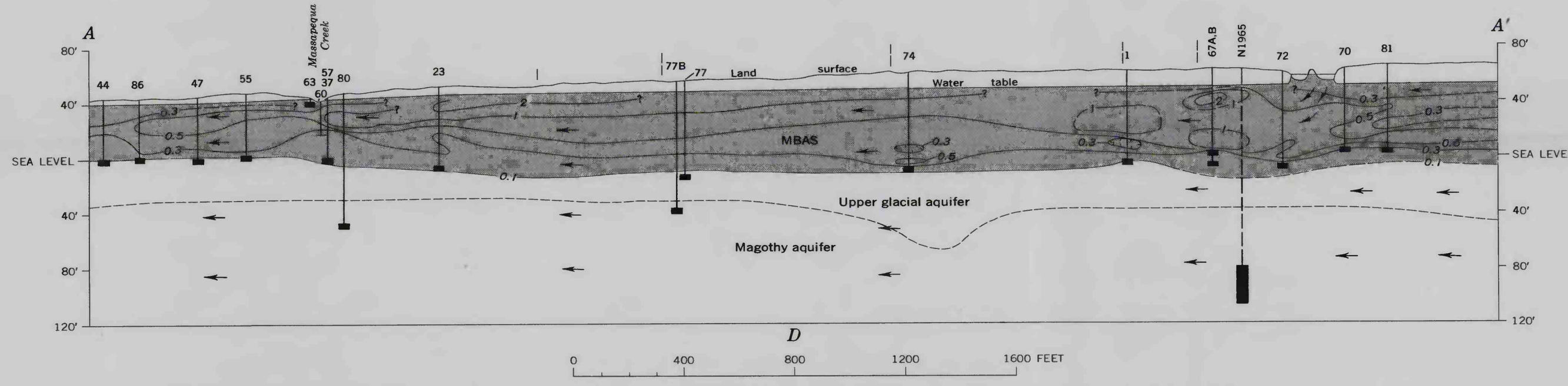
HYDROGEOCHEMICAL SECTION A-A' SHOWING THE DIRECTION OF GROUND-WATER FLOW AND GEOLOGIC UNITS (A) AND DISTRIBUTION OF HEXAVALENT CHROMIUM (B), CADMIUM, (C), AND MBAS (D) ALONG THE LONGITUDINAL AXIS OF THE PLUME CONTAINING PLATING WASTES, SOUTH FARMINGDALE AREA, NASSAU COUNTY, NEW YORK
