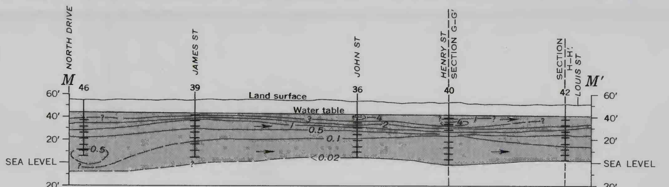
HYDROGEOCHEMICAL SECTIONS SHOWING THE DISTRIBUTION OF MBAS IN THE UPPER GLACIAL AQUIFER TRANSVERSE (B-B' TO L-L') AND PARALLEL (M-M') TO THE DIRECTION OF GROUND-WATER FLOW SOUTH FARMINGDALE AREA, NASSAU COUNTY, NEW YORK
