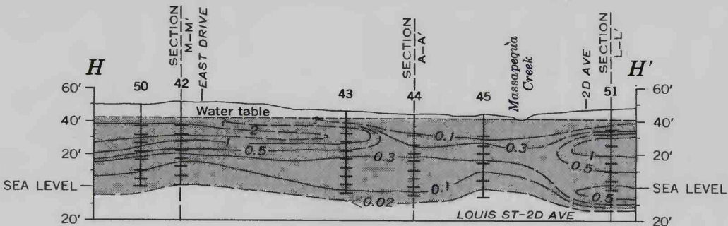
HYDROGEOCHEMICAL SECTIONS SHOWING THE DISTRIBUTION OF MBAS IN THE UPPER GLACIAL AQUIFER TRANSVERSE (B-B' TO L-L') AND PARALLEL (M-M') TO THE DIRECTION OF GROUND-WATER FLOW SOUTH FARMINGDALE AREA, NASSAU COUNTY, NEW YORK
