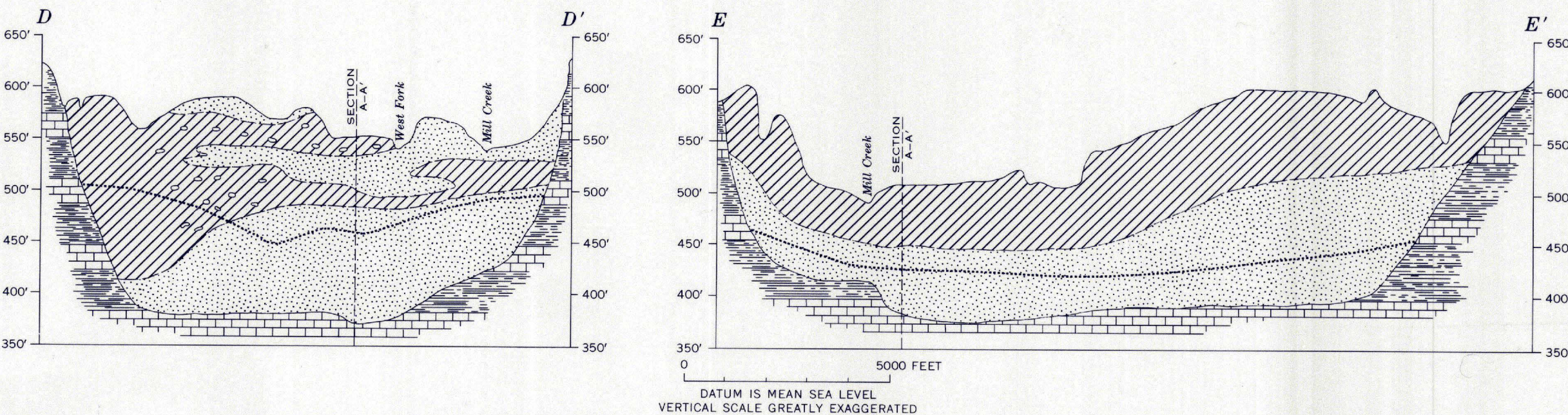
GENERALIZED GEOLOGIC SECTIONS, MILL CREEK VALLEY, BUTLER AND HAMILTON COUNTIES, OHIO
