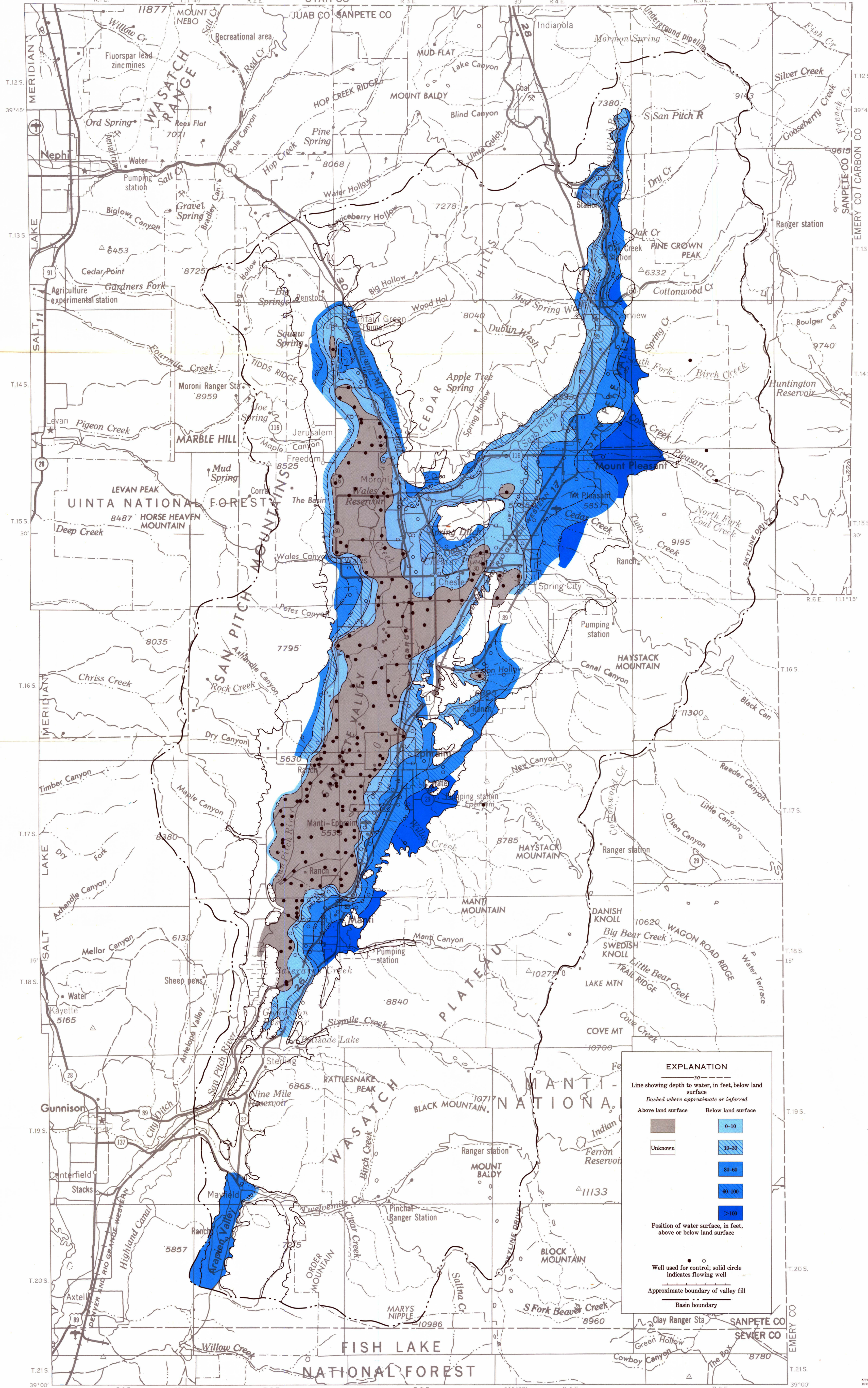
POSITION OF THE GROUND-WATER SURFACE DURING NOVEMBER AND DECEMBER 1966
