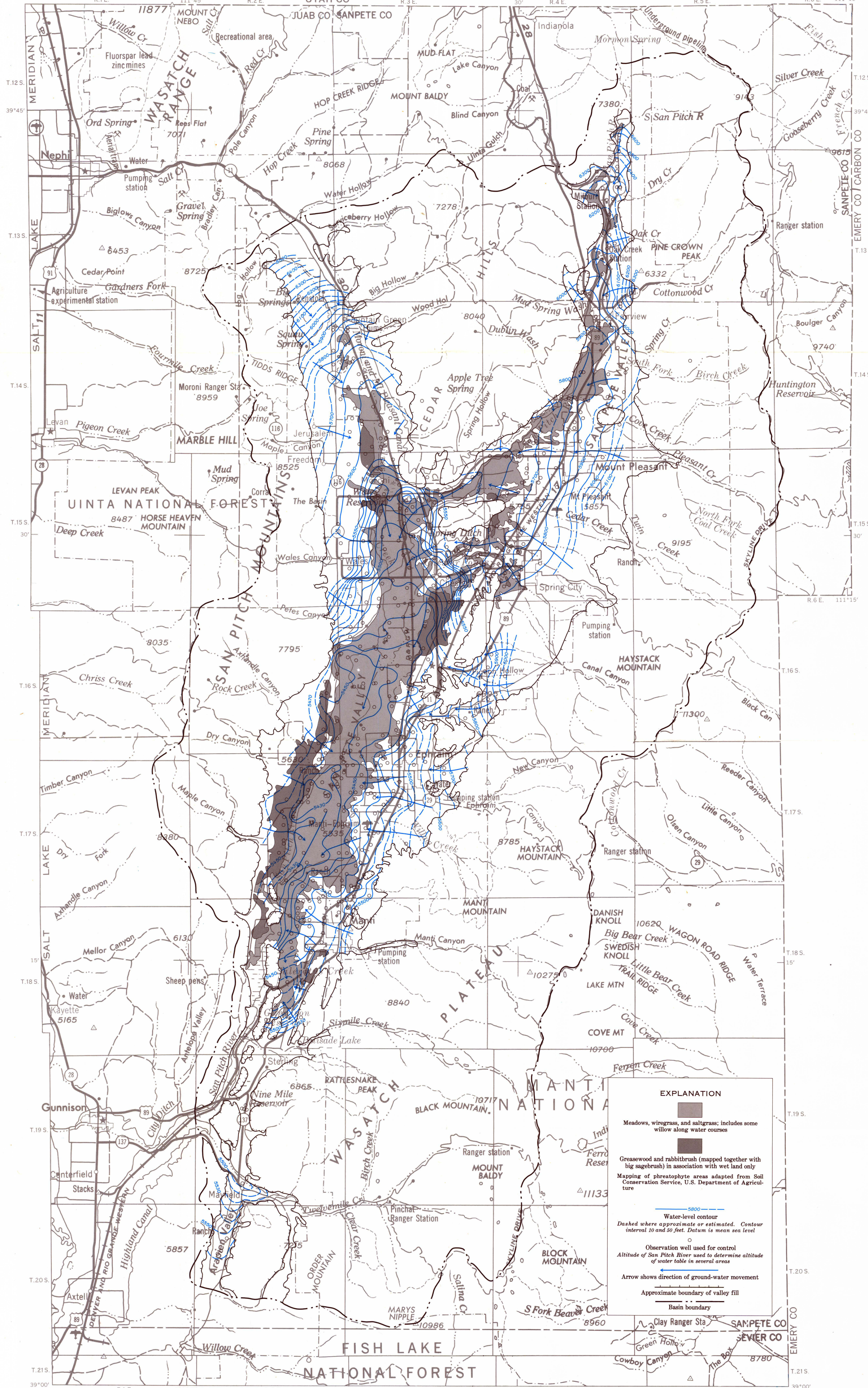
WATER-LEVEL CONTOURS DURING NOVEMBER AND DECEMBER 1966 AND PHREATOPHYTE AREAS
