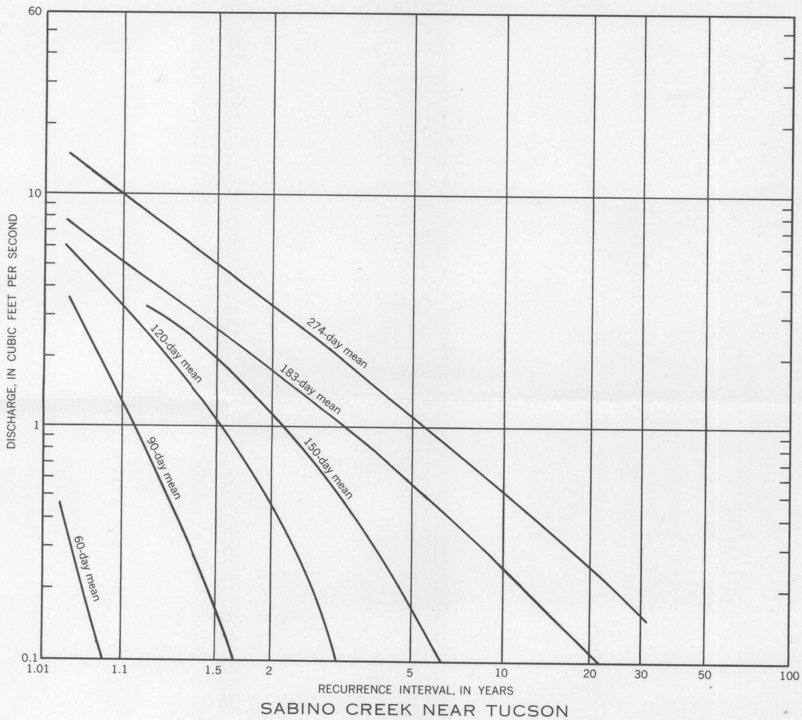
GRAPHS SHOWING LOW-FLOW FREQUENCY CURVES FOR STREAMS IN THE UPPER SANTA CRUZ RIVER BASIN, SANTA CRUZ AND PIMA COUNTIES, ARIZONA
