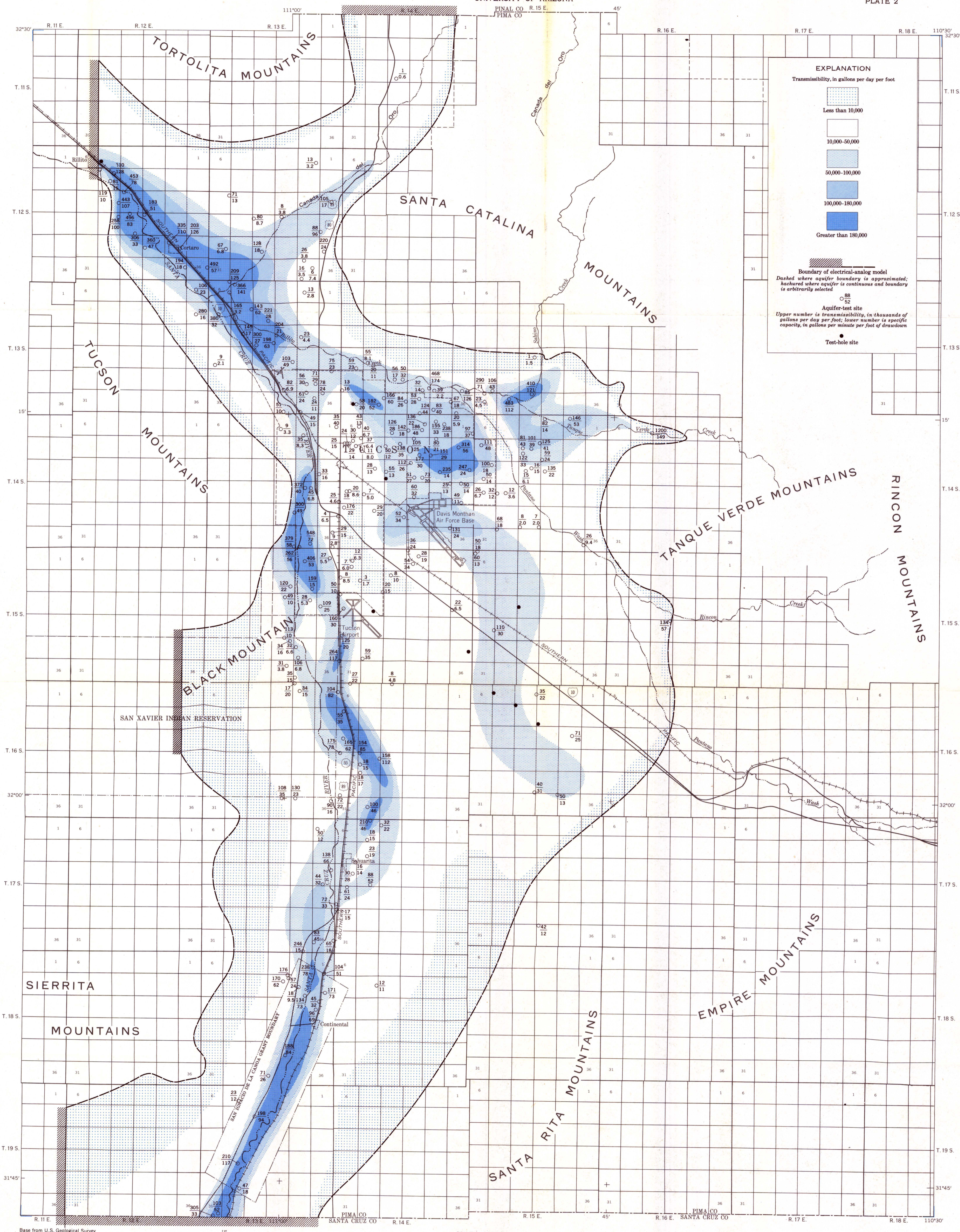
MAP SHOWING GENERALIZED TRANSMISSIBILITY PATTERN USED IN ELECTRICAL-ANALOG MODEL, TUCSON BASIN, SOUTHEASTERN ARIZONA
