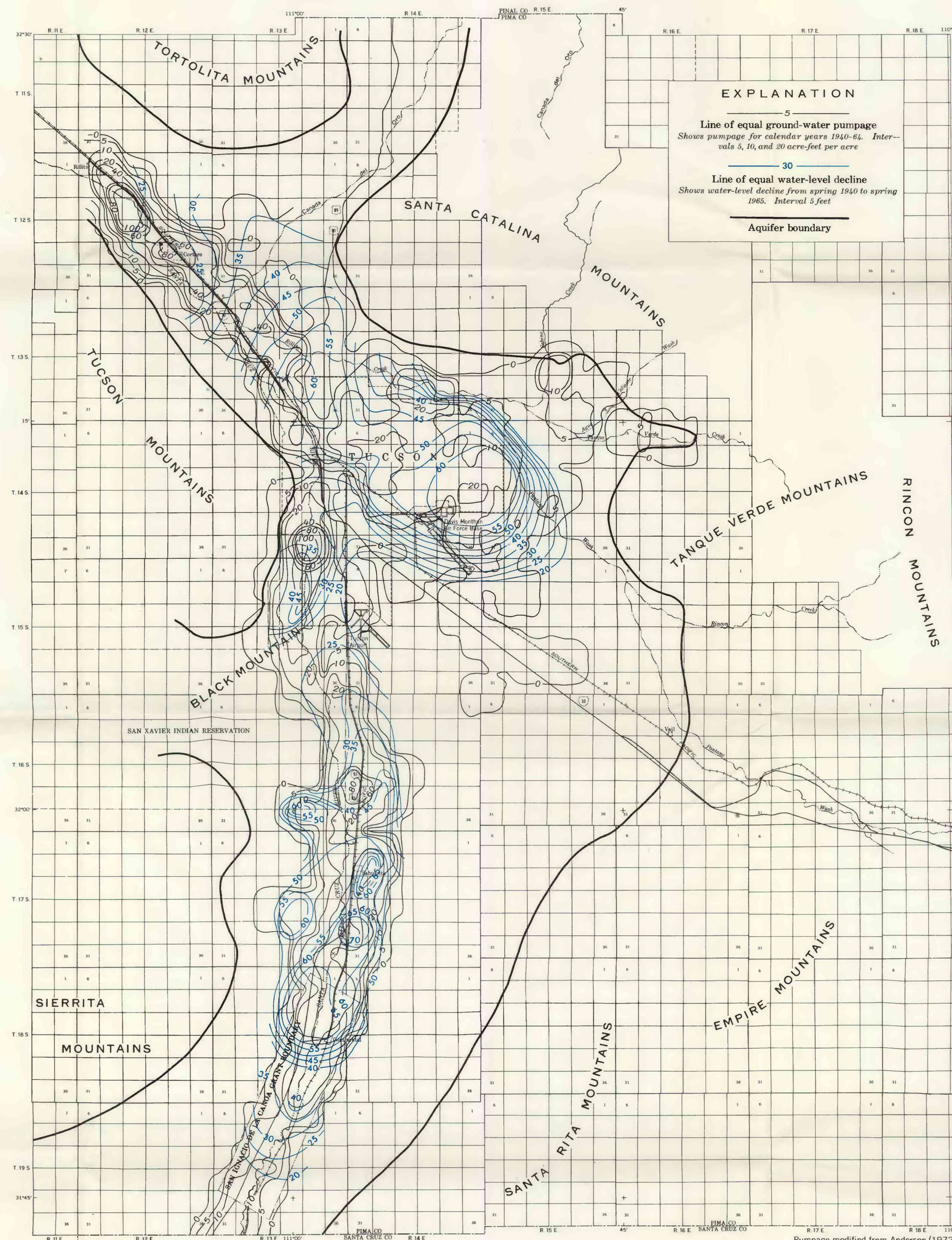
B. PUMPAGE AND WATER-LEVEL DECLINES, 1940-65
