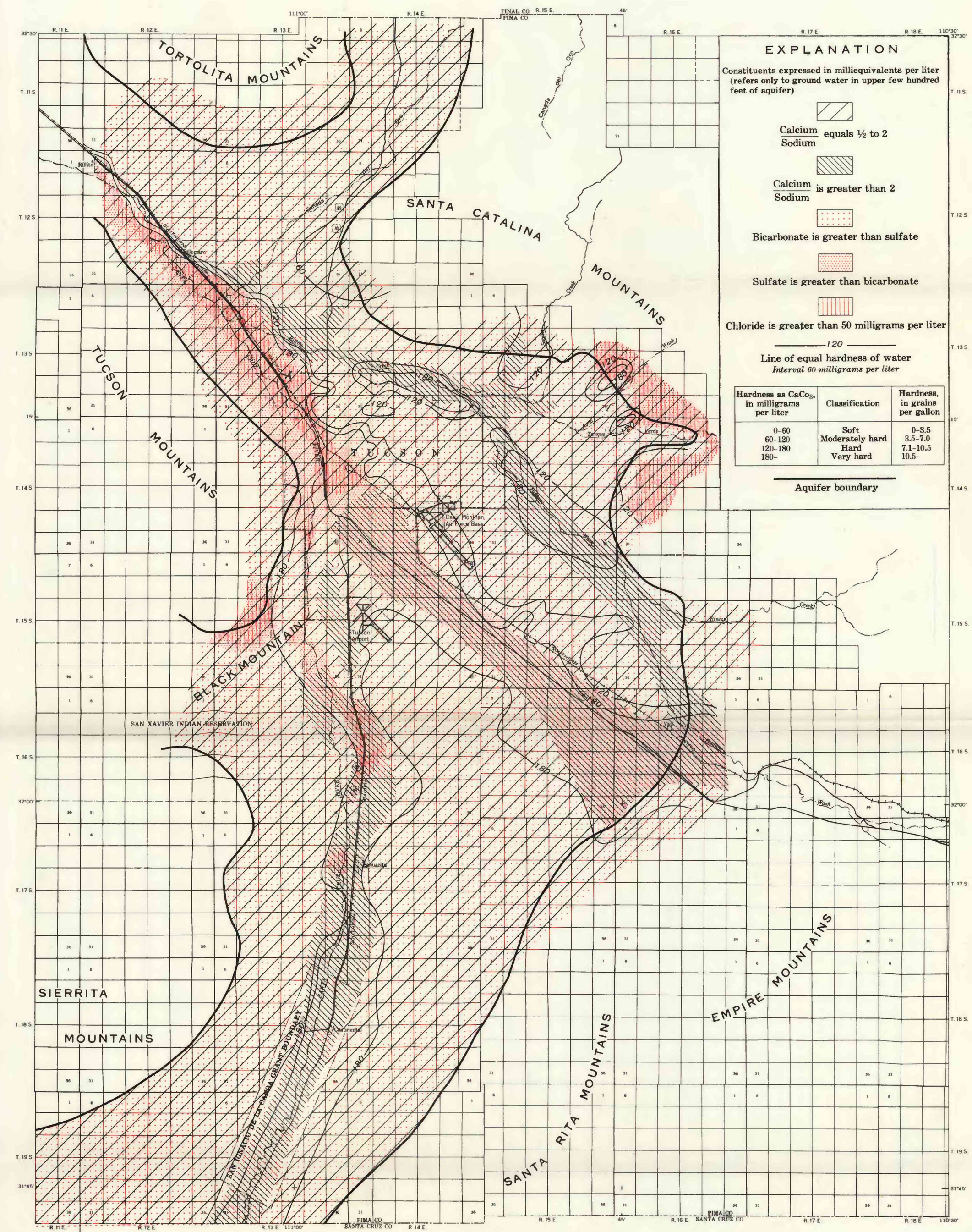
B. MAJOR IONS AND HARDNESS IN SHALLOW GROUND WATER
