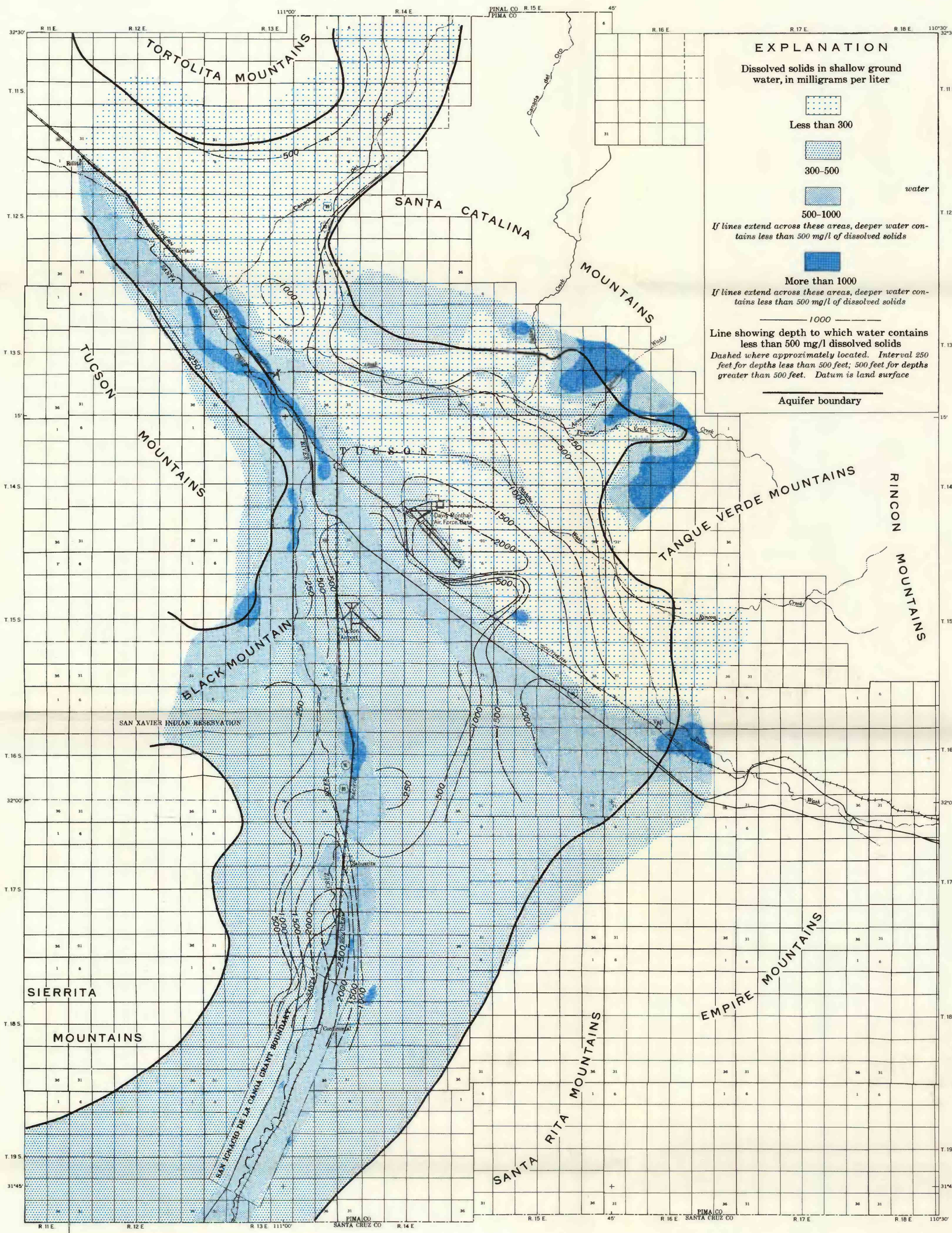
A. AREAL DISTRIBUTION OF DISSOLVED SOLIDS IN SHALLOW GROUND WATER AND DEPTH TO WHICH GROUND WATER CONTAINS LESS THAN 500 MILLIGRAMS PER LITER OF DISSOLVED SOLIDS
