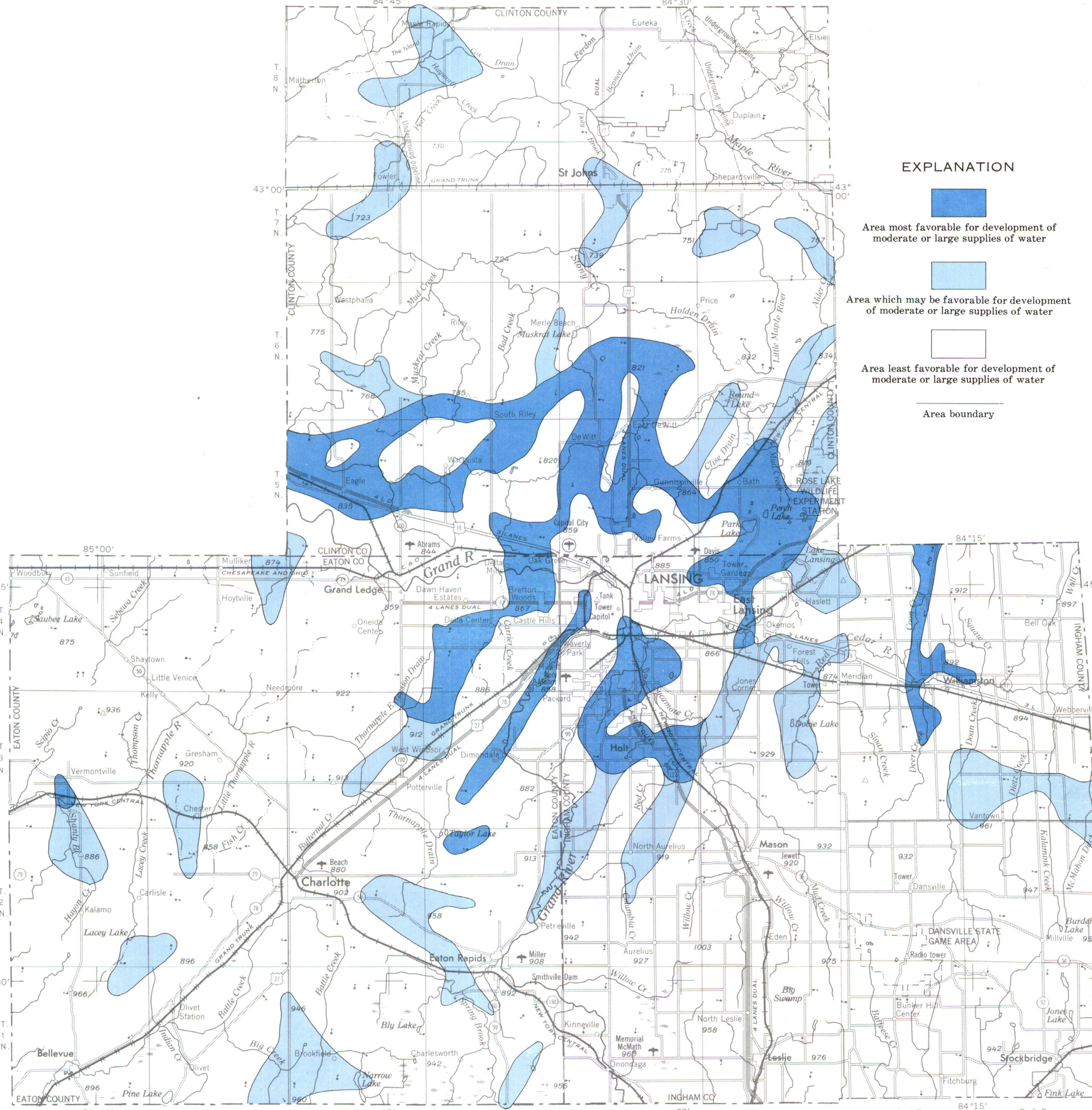
D. BURIED DEPOSITS OF OUTWASH SOME OF WHICH ARE FAVORABLE SOURCES FOR WATER SUPPLIES. ARE SCATTERED THROUGHOUT THE REGION
