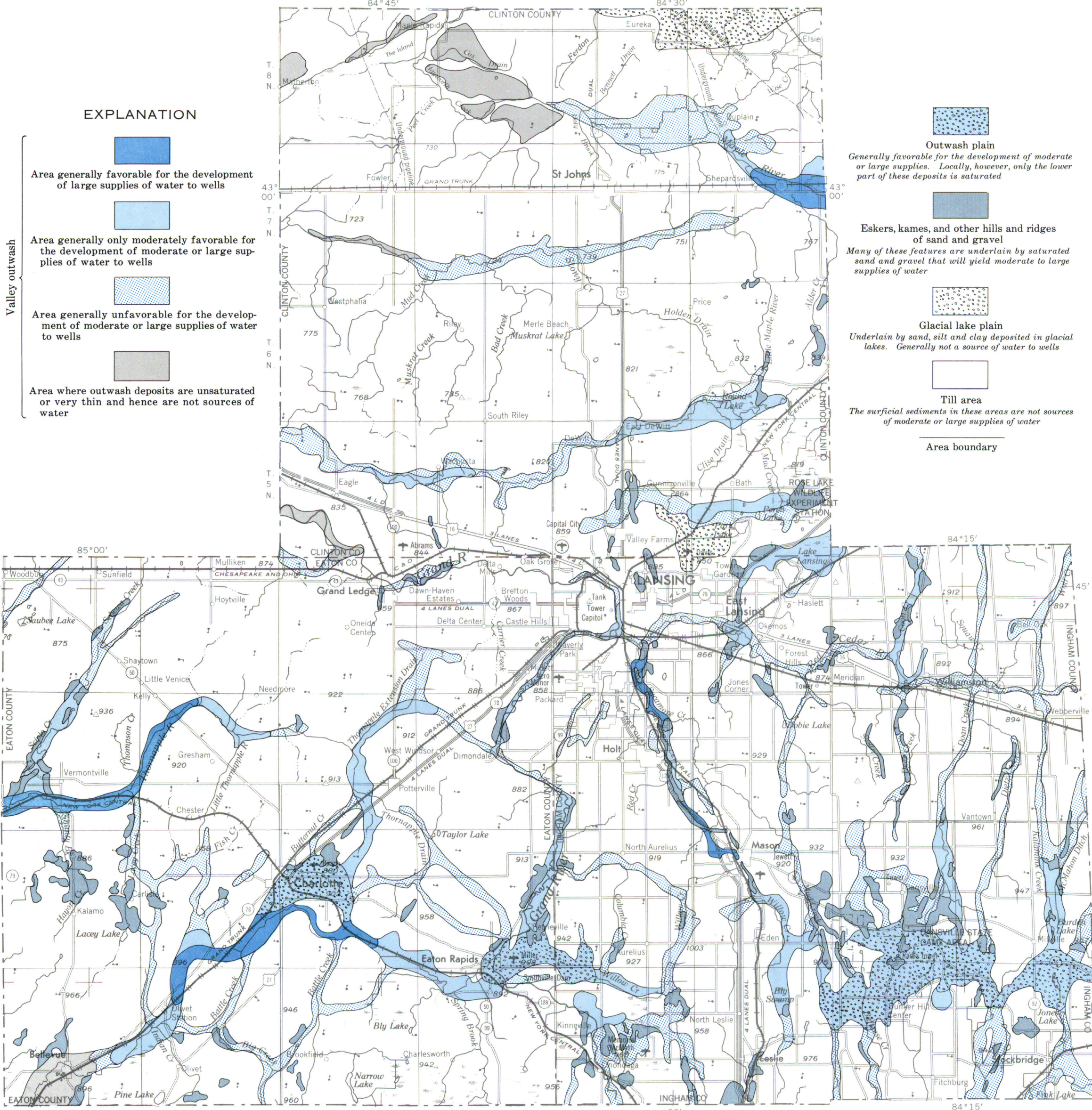
C. THE POTENTIAL FOR DEVELOPMENT OF WATER SUPPLIES FROM GLACIAL DEPOSITS VARIES GREATLY THROUGHOUT THE REGION
