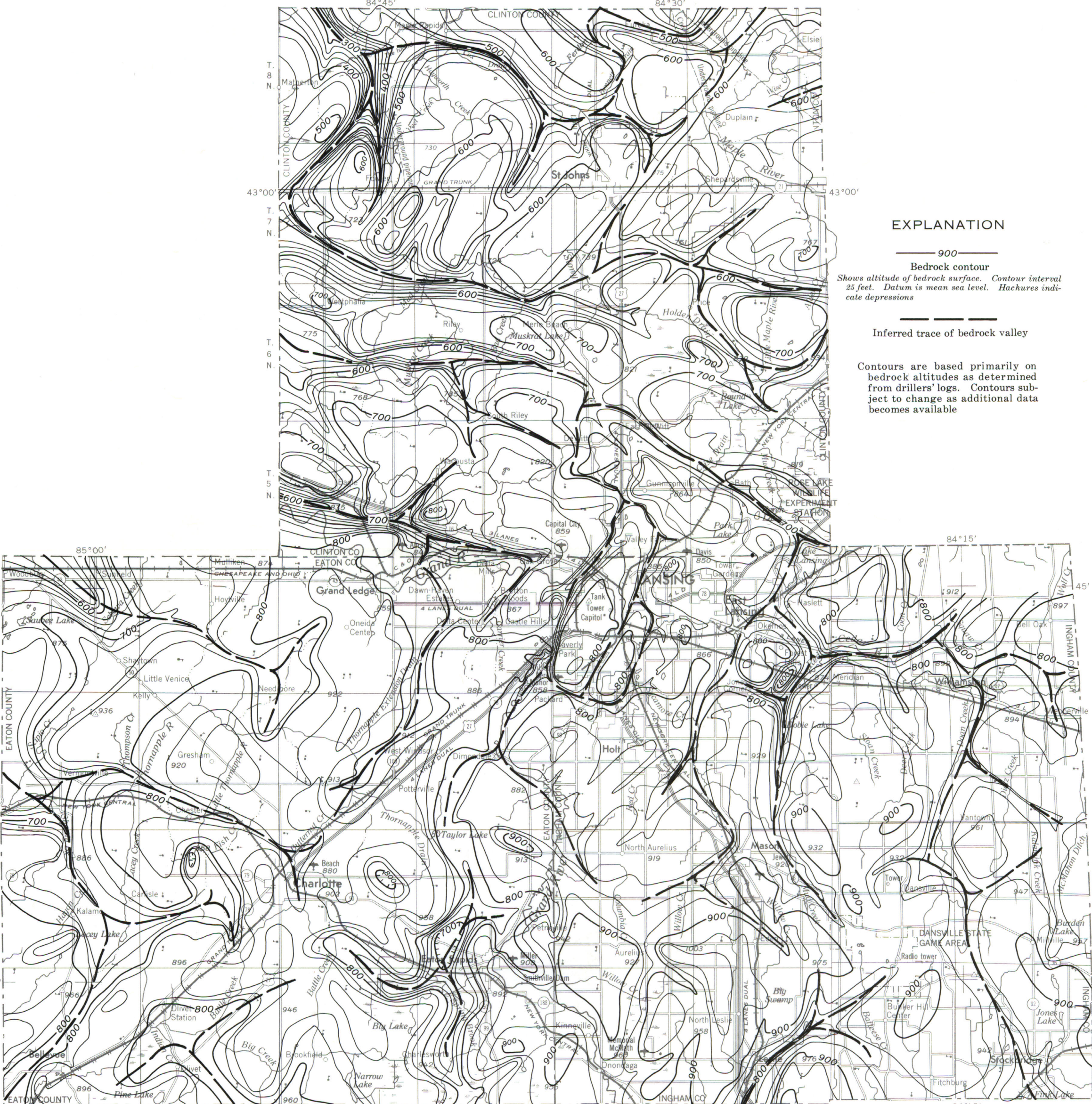
A. THE ALTITUDE OF THE BEDROCK SURFACE RANGES FROM LESS THAN 300 FEET TO MORE THAN 900 FEET
