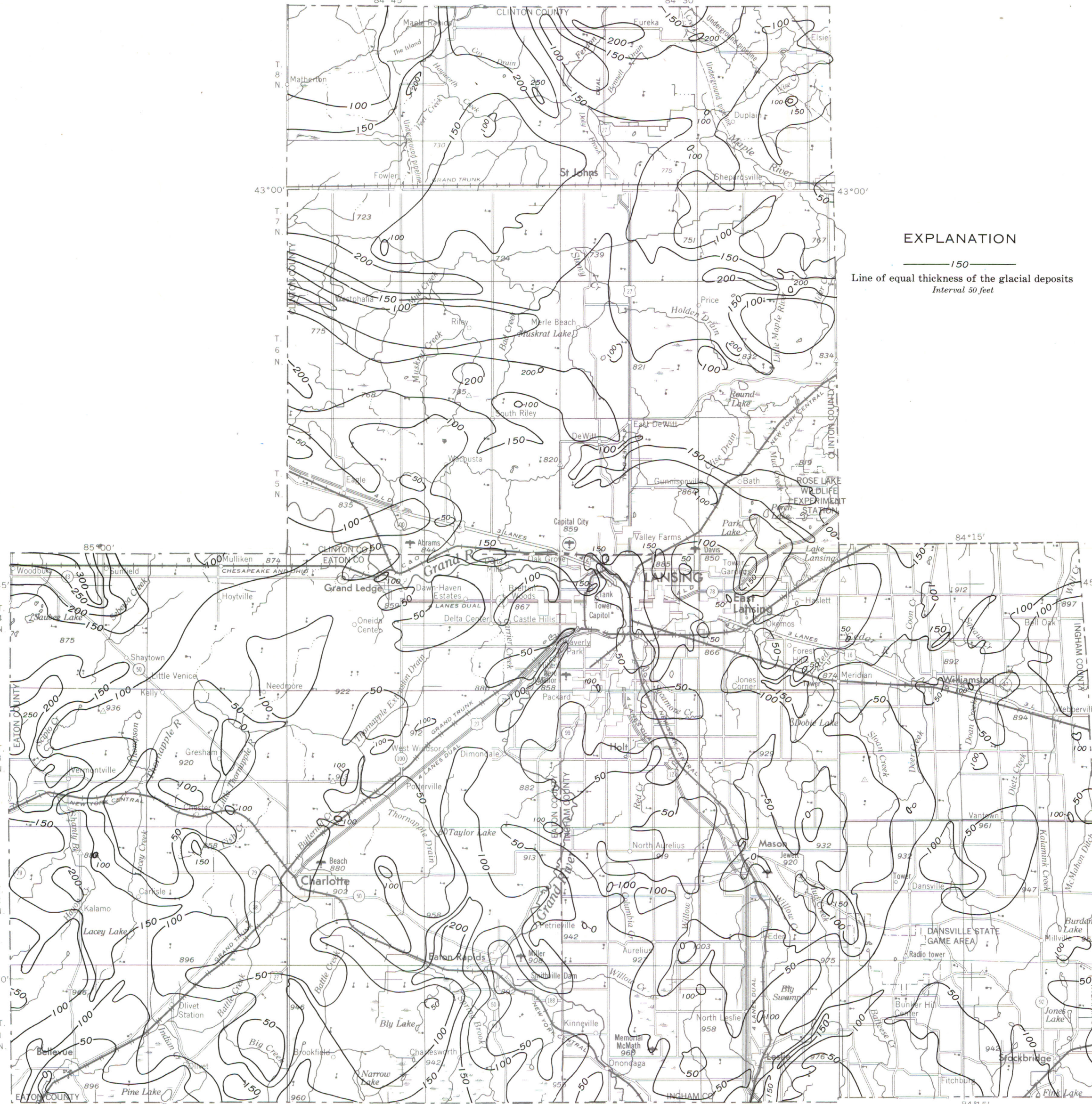
B. THE THICKNESS OF THE GLACIAL DEPOSITS RANGES BETWEEN 50 AND 200 FEET IN MOST OF THE REGION
