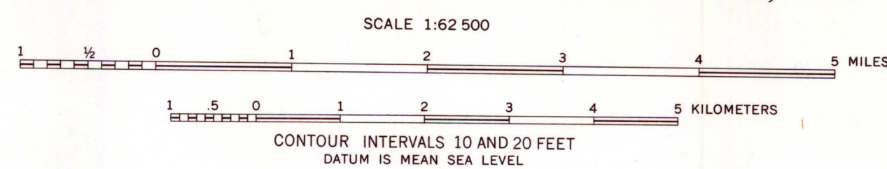
MAP SHOWING STREAMFLOW IN KALAMAZOO COUNTY, SOUTHWESTERN MICHIGAN
