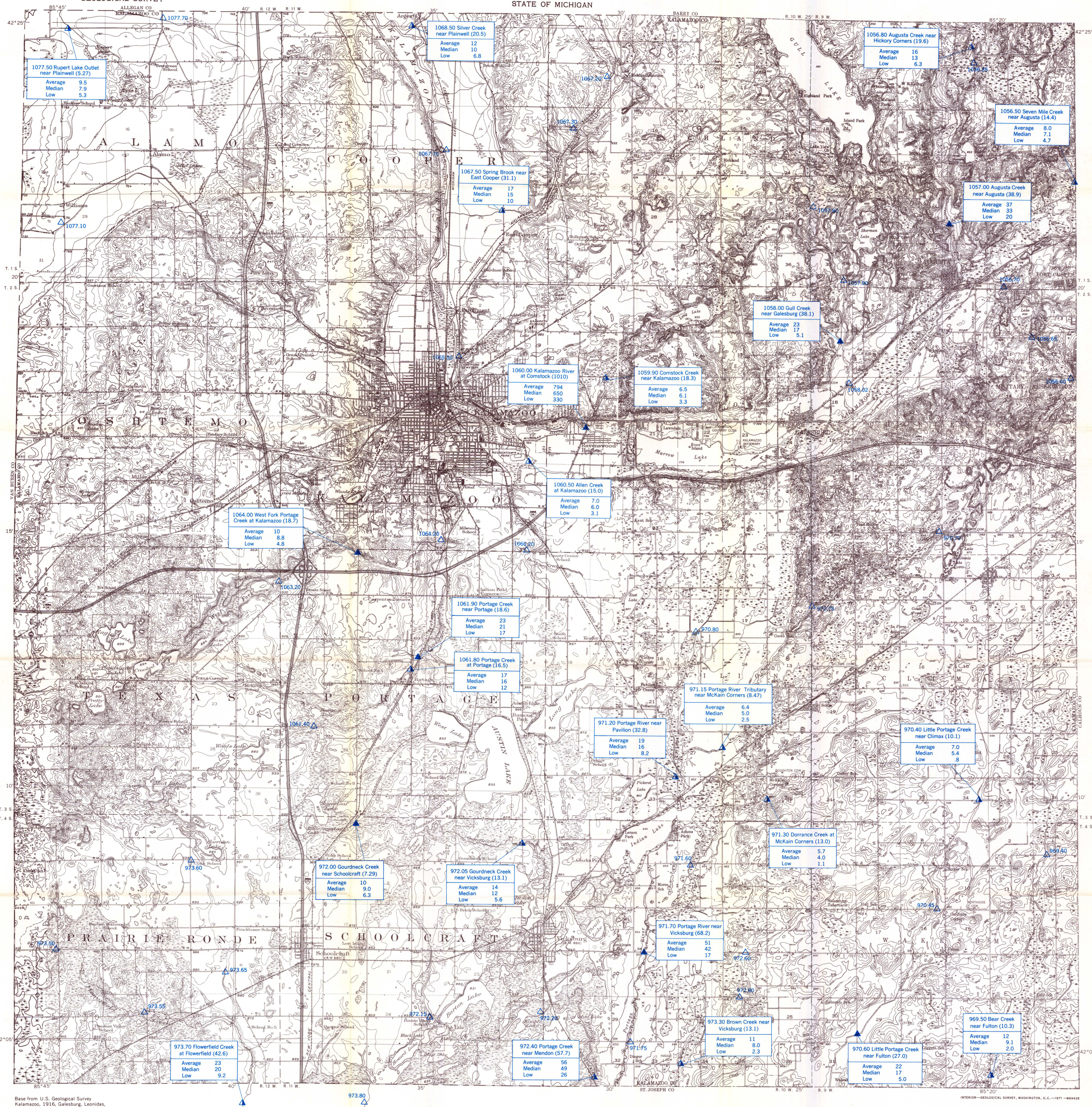
MAP SHOWING STREAMFLOW IN KALAMAZOO COUNTY, SOUTHWESTERN MICHIGAN
