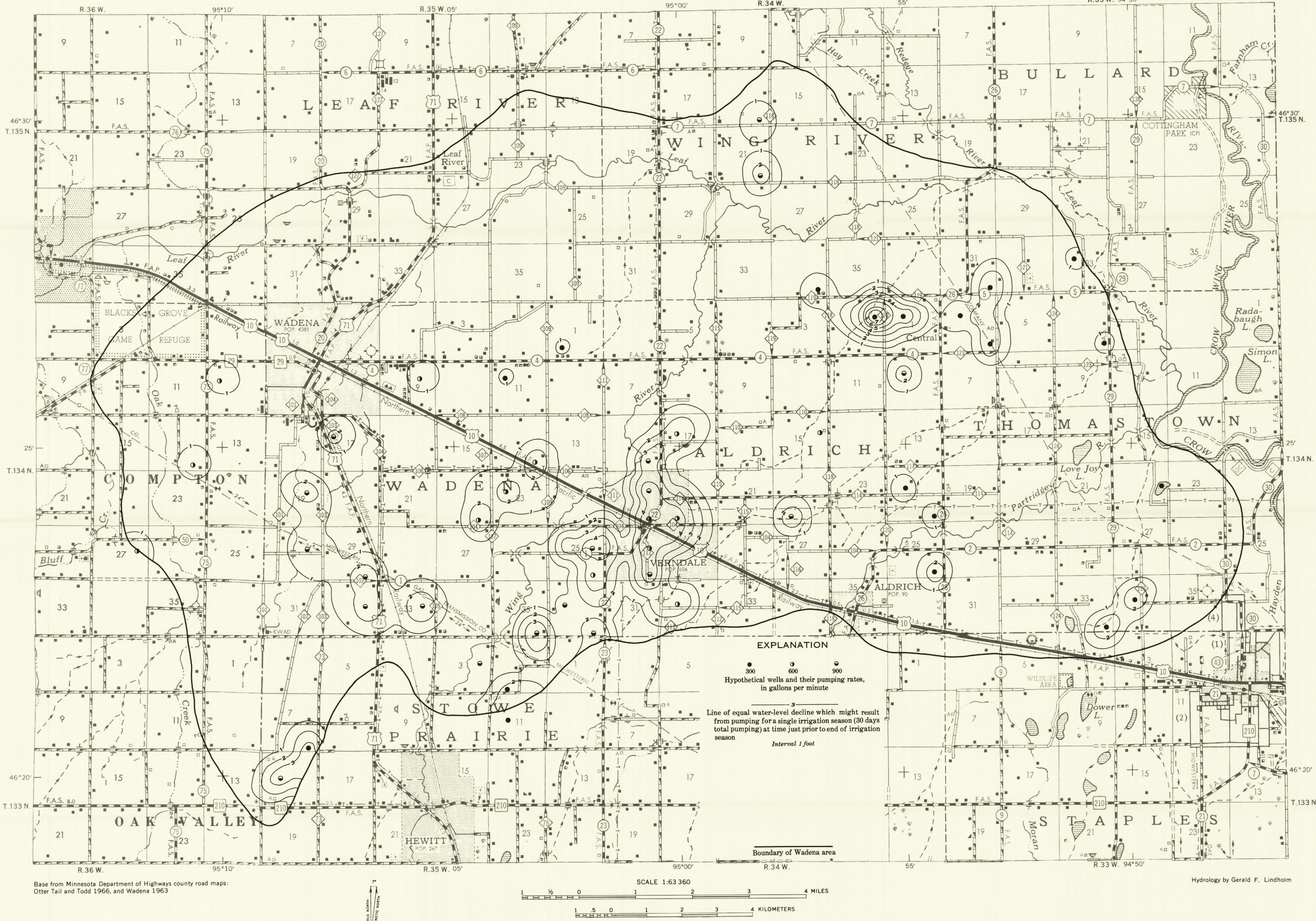
MAP SHOWING THEORETICAL WATER-LEVEL DECLINE THAT MIGHT RESULT FROM PUMPING A HYPOTHETICAL 5-YEAR DEVELOPMENT PLAN IN THE WADENA AREA, CENTRAL MINNESOTA
