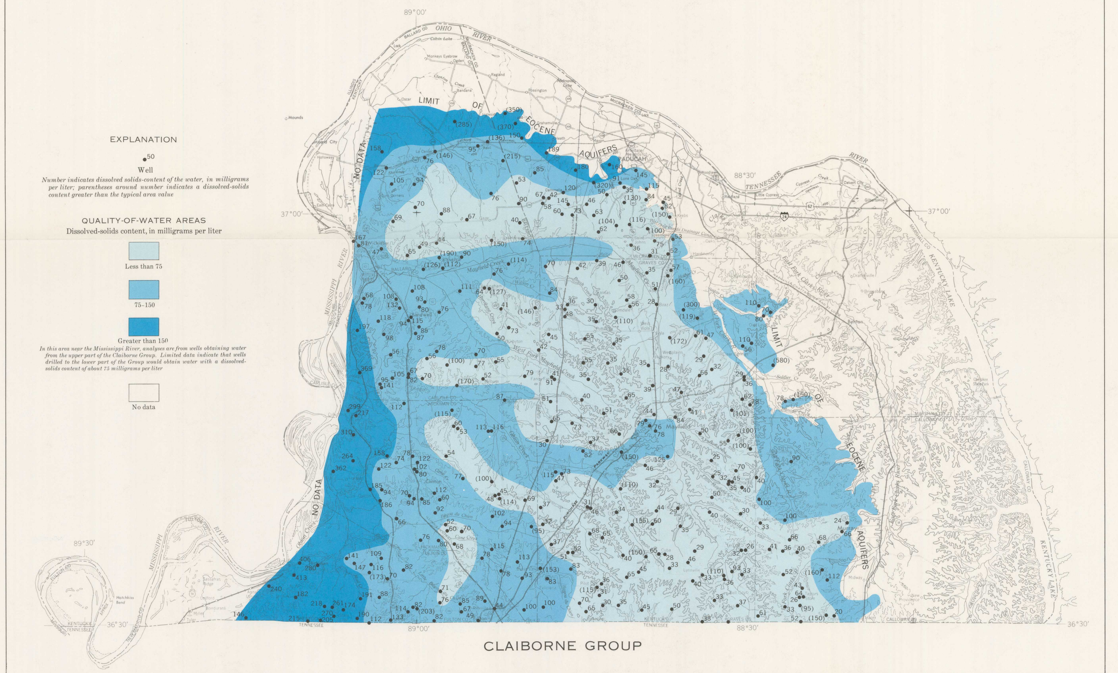
MAPS SHOWING DISSOLVED-SOLIDS CONTENT OF WATER FROM MC NAIRY FORMATION AND THE CLAIBORNE GROUP, JACKSON PURCHASE REGION, KENTUCKY
