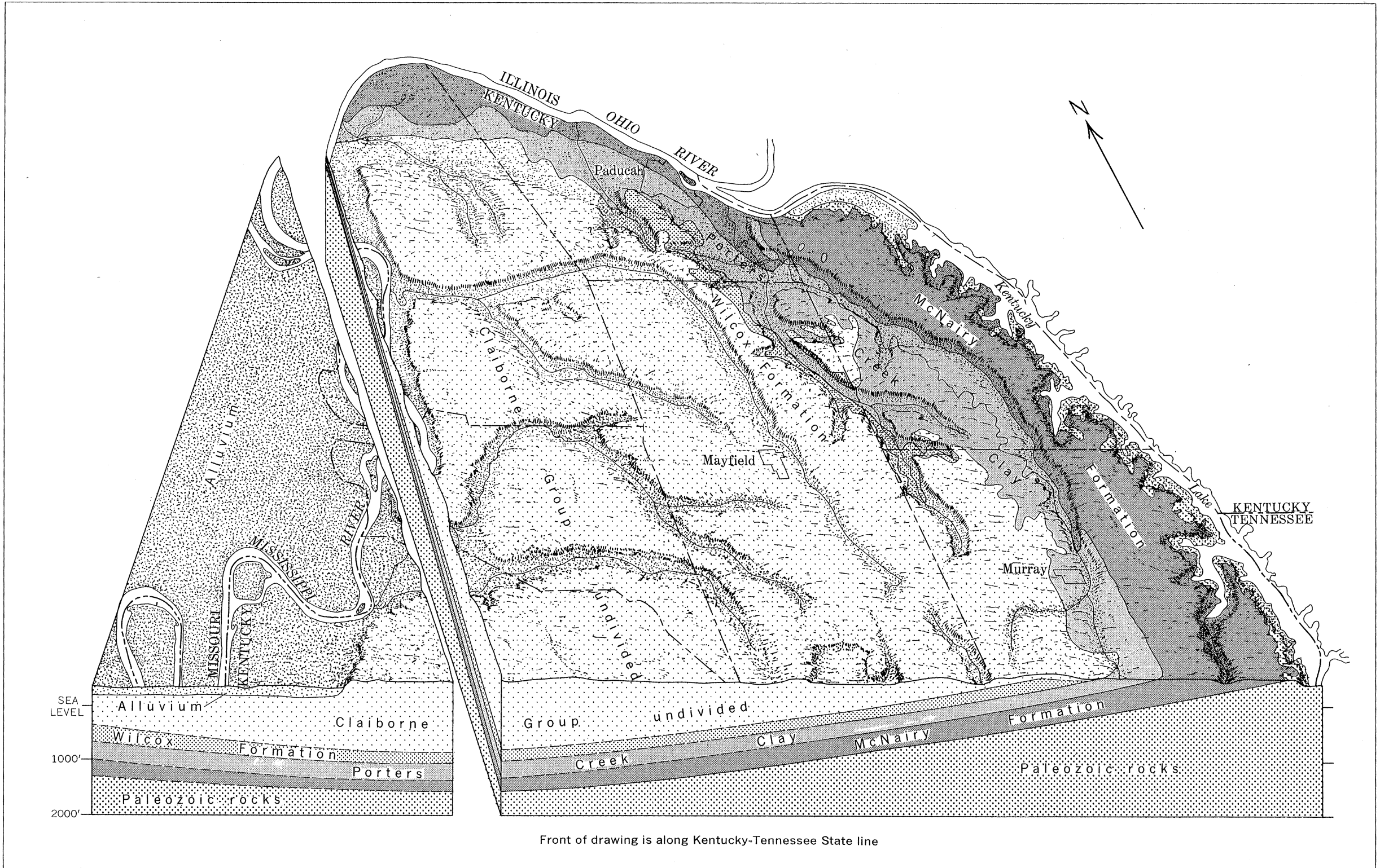
BLOCK DIAGRAM SHOWING THE GENERALIZED STRATIGRAPHY AND STRUCTURE OF THE JACKSON PURCHASE REGION, KENTUCKY
