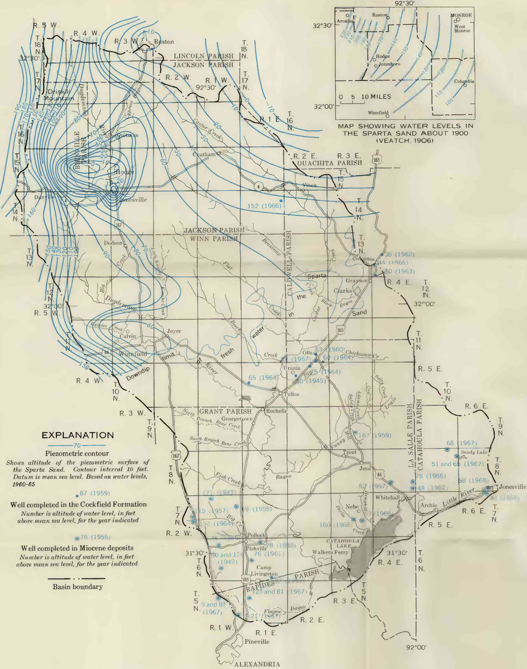
ALTITUDE OF WATER LEVELS IN THE SPARTA SAND, COCKFIELD FORMATION, AND MIOCENE DEPOSITS
