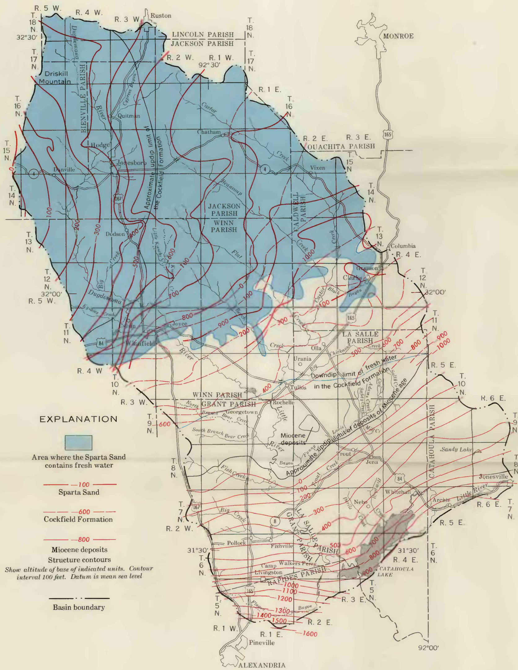
ALTITUDE OF THE BASE OF THE SPARTA SAND, COCKFIELD FORMATION, AND MIOCENE DEPOSITS
