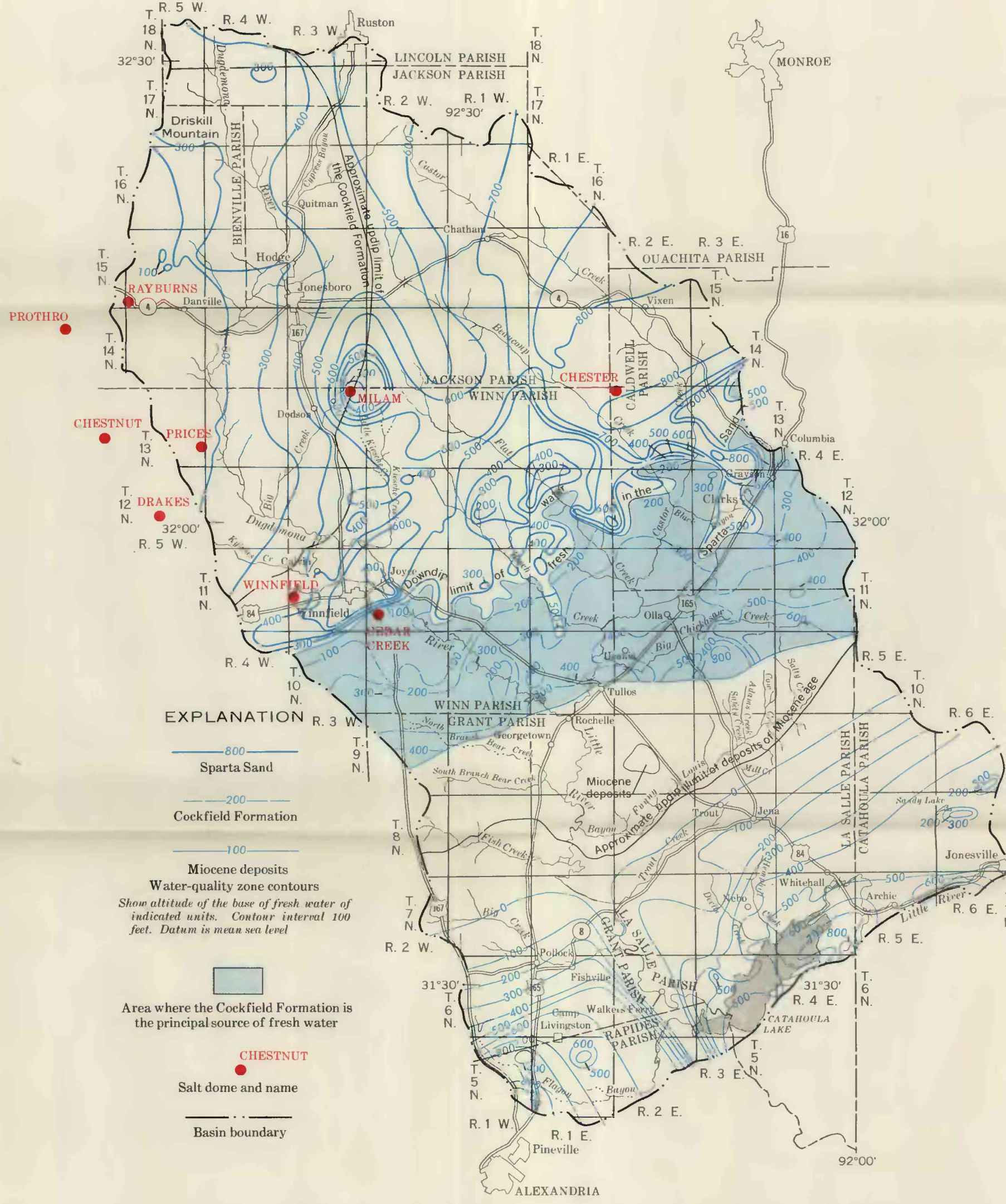
ALTITUDE OF THE BASE OF FRESH GROUND WATER
